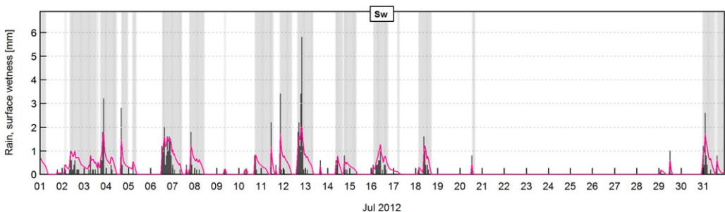
Fig. 16. Rainfall (bars), modelled surface wetness (pink lines) and observed wetness state (shading indicates wet periods) for July 2012 at Swindon. (For interpretation of the references to colour in this figure legend, the reader is referred to the web version of this article.)
