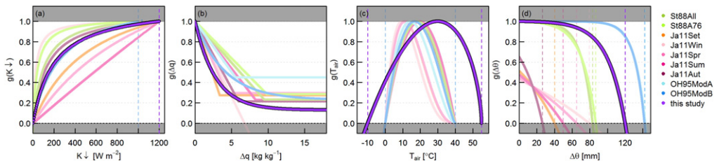
Fig. A1. Relations for the dependence of surface conductance on (a) incoming shortwave radiation K_d , (b) specific humidity deficit \Delta q , (c) air temperature T_{air} and (d) soil moisture deficit \Delta\theta for this study and from literature (St88 - Stewart (1988): all data (All) and 1976 data only (A76); OH95 - Ogink-Hendriks (1995): linear dependence on \Delta q (ModA) and exponential dependence on \Delta q (ModB); Ja11 - Järvi et al. (2011): recommended values based on the whole data set (Set) and for each season separately (Win, Spr, Sum, Aut)).
