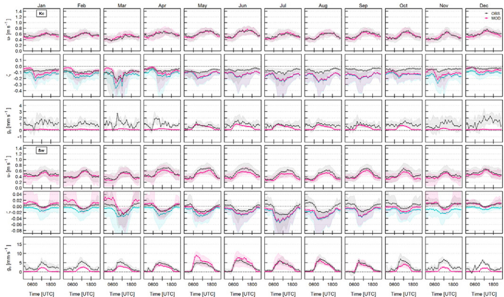
Fig. 11. Median diurnal cycle and inter-quartile range by month for modelled (pink) and observed (grey) friction velocity u_* ; stability parameter \zeta calculated from (z_m - z_d) / L_{oh MOD} or (z_m - z_d) / L_{oh OBS} ; and, for dry conditions only, surface conductance g_s . For \zeta , results are also shown (in cyan) for the case where the OHM coefficients are kept constant throughout the year (MOD cc ). Note different y-axis scales ( \zeta and g_s ) for Kc and Sw. (For interpretation of the references to colour in this figure legend, the reader is referred to the web version of this article.)
