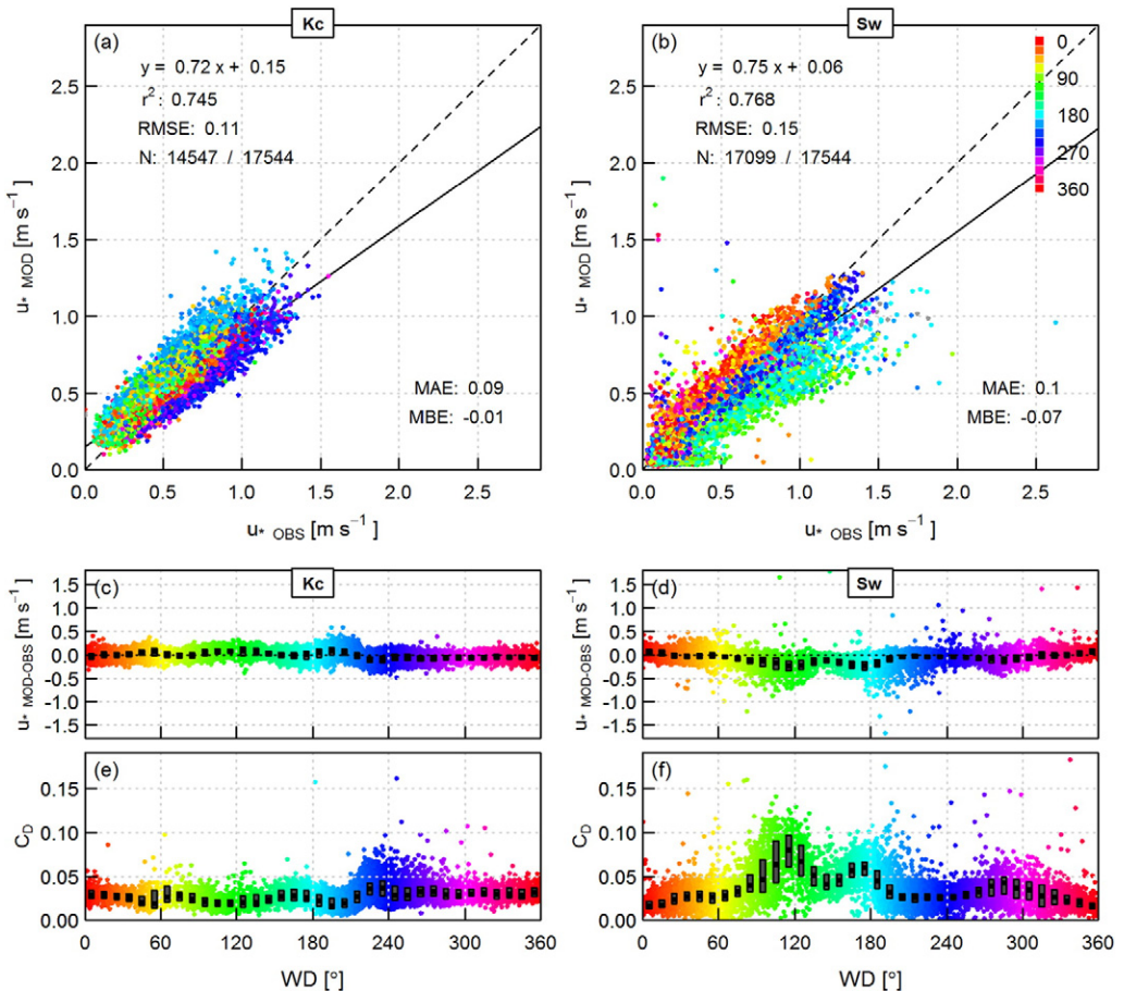
Fig. 10. (a, b) Modelled versus observed friction velocity coloured according to wind direction; (c, d) difference between modelled and observed friction velocity as a function of wind direction; (e, f) observed drag coefficient C_D = (u_*/U)^2 in near-neutral conditions ( -0.1 < \zeta < 0.1 ) as a function of wind direction. Boxplots indicate the median and inter-quartile range for bins of 10^\circ . (For interpretation of the references to colour in this figure legend, the reader is referred to the web version of this article.)
