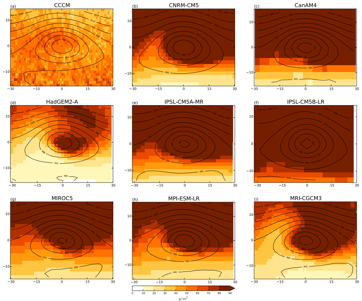
FIG. 8. LWP around cyclone centers over the Southern Ocean in austral summer (DJF). Cyclone composites calculated using the method of Field and Wood (2007): (a) CCCM data and (b)–(i) CMIP5 AMIP experiments.
