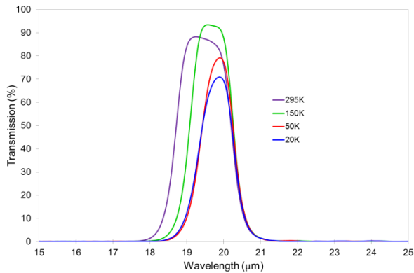
Fig 7. Cooled 20 μm 8.0% FWHM wide-bandpass filter at 295K, narrowing to 5.2% at 20K on CdTe
