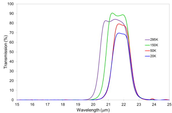
Fig 8. Cooled 22 μm 9.4% FWHM wide-bandpass filter at 295K, narrowing to 6.0% at 20K on CdTe
