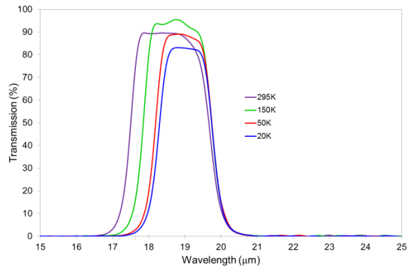
Fig 6. Cooled 19 μm 12.0% FWHM wide-bandpass filter at 295K, narrowing to 8.1% at 20K on CdTe
