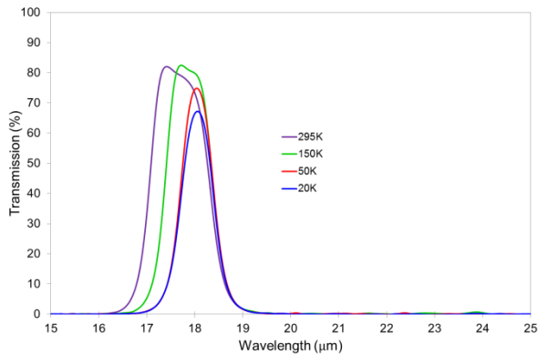
Fig 5. Cooled 18 μm 7.2% FWHM wide-bandpass filter at 295K, narrowing to 4.2% at 20K on CdTe
