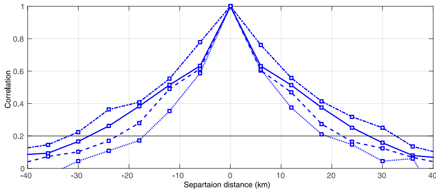
FIG. 5. Horizontal observation correlations for elevation 2° at heights 1.1 km (dotted), 2.7 km (dashed), 3.5 km (solid), and 4.3 km (dot-dashed) for case 1 (control). Error correlations are deemed to be insignificant below the horizontal line at 0.2.
