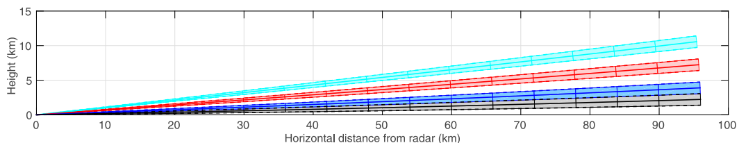
FIG. 2. A typical radar beam at elevations 1° (black), 2° (blue), 4° (red), and 6° (cyan).
