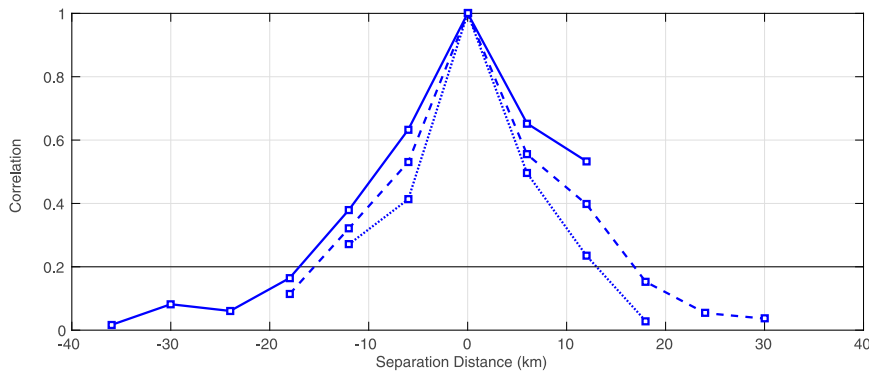
FIG. 9. Along-beam observation correlations for elevation 2° at heights 1.1 km (dotted), 3.0 km (dashed), and 3.5 km (solid) for case 1 (control).
