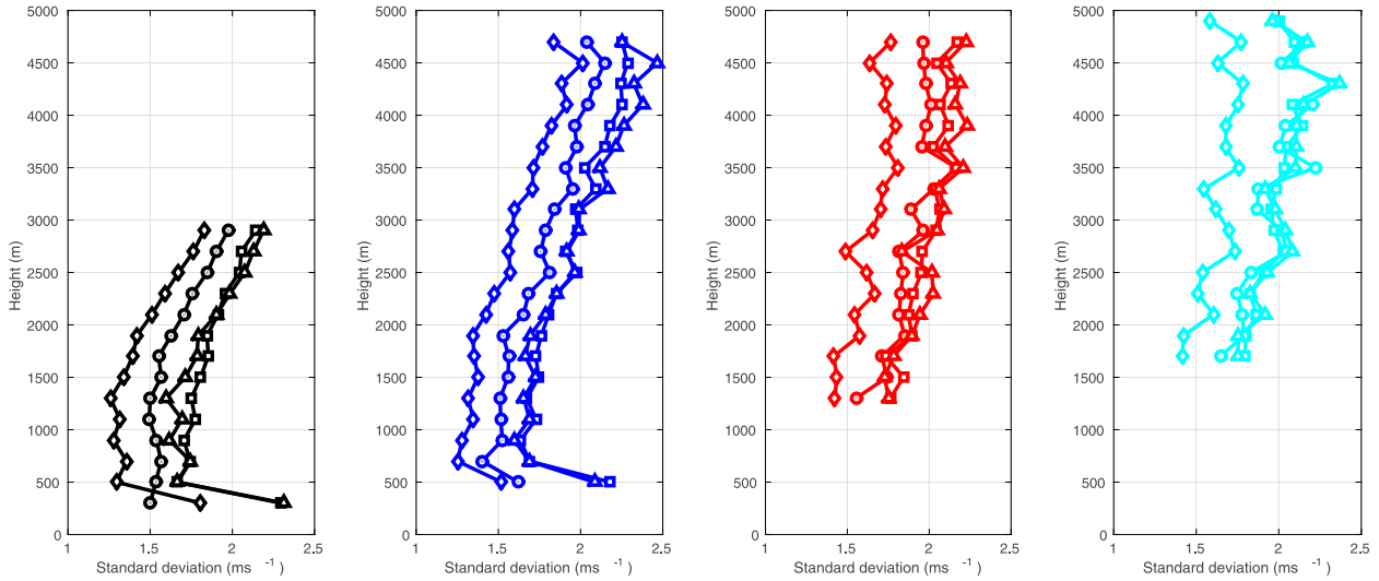
FIG. 4. Horizontal observation error standard deviation for elevations 1° (black), 2° (blue), 4° (red), and 6° (cyan) for case 1 (control; squares), case 2 (alternate background error statistics; diamonds), case 3 (thinned raw data; triangles) and case 4 (new observation operator; circles).
