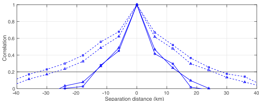
FIG. 12. Horizontal observation correlations for elevation 2^\circ at a range of 24 km (solid) and 90 km (dashed) for case 1 (control; squares) and case 3 (thinned raw data; triangles). Error correlations are deemed to be insignificant below the horizontal line at 0.2.
