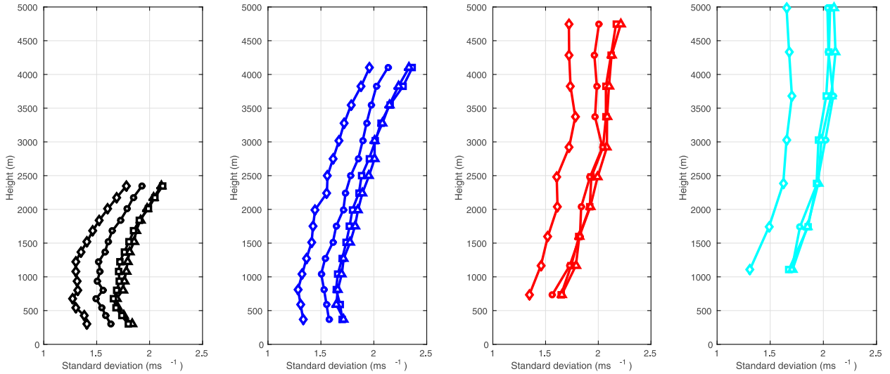
FIG. 8. Along-beam observation error standard deviation for elevations 1° (black), 2° (blue), 4° (red), and 6° (cyan) for case 1 (control; squares), case 2 (alternate background error statistics; diamonds), case 3 (thinned raw data; triangles), and case 4 (new observation operator; circles).
