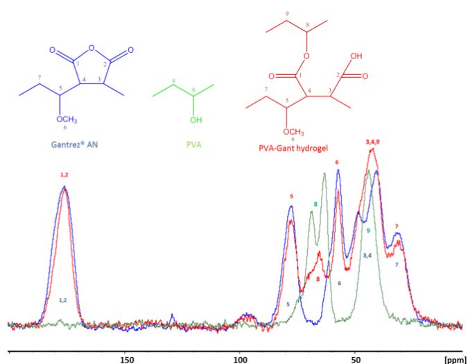
Fig. 2. Solid state 13 C CP-MAS NMR spectra of Gant, PVAm and PVAm - Gant (1:1) hydrogel sample.
