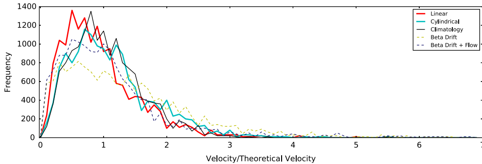
Figure 5. Histogram showing the ratio of observed to predicted IMD propagation velocities for each of the five models discussed in the text calculated for all timesteps present in the dataset. Thick lines represent our linear and cylindrical models respectively; thin black represents a simple model based on the climatology; dashed lines represent a simple beta drift model (not) including background monsoonal flow.
