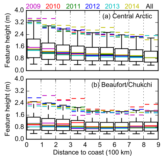
Figure 10. Surface feature height, h_f , as a function of distance to the nearest coastline within the (a) Central Arctic and (b) Beaufort/Chukchi regions (given in Fig. 5), presented using box and whisker plots (5, 25, 50, 75, 95 percentiles). The coastline distance bin width is 100 km. The black boxes (and whiskers) show the results from all features detected in each region, while the colours represent the results from each year.
