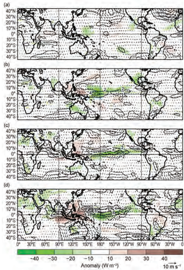
FIG. 4.4. Anomalous 850-hPa wind vectors and speed (contour interval is 2 \text{ m s}^{-1} ) and anomalous OLR (shaded, \text{W m}^{-2} ) during (a) DJF 2014/15, (b) MAM 2015, (c) JJA 2015, and (d) SON 2015. Anomalies are departures from the 1981–2010 period monthly means.
