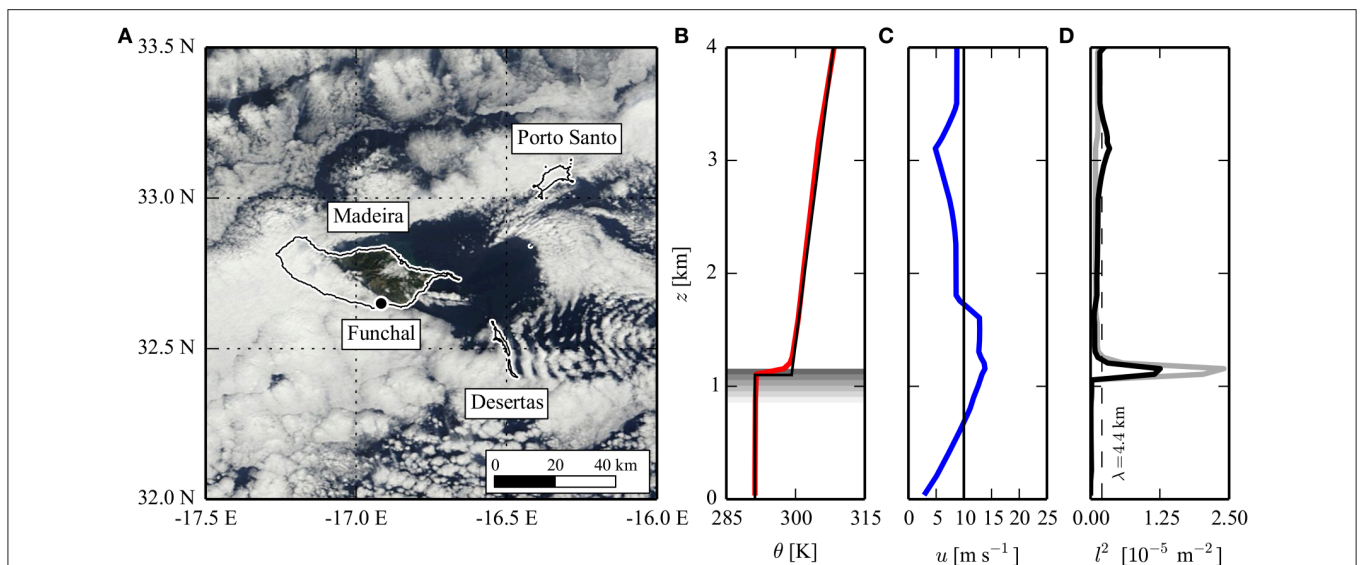
FIGURE 2 | (A) MODIS Terra visible satellite image on 24 December 2013, showing signature of trapped lee waves downwind of the Desertas islands in the Madeira archipelago. Coastlines are shown with solid white-black contours. The location of the sounding site (Funchal) is marked with a black dot. Flow is from left to right. Satellite image from NASA Earthdata and SRTM topography data from Jarvis et al. (2008). (B–D) Funchal operational sounding at 1200 UTC 24 December 2013. The panels show vertical profiles of (B) potential temperature, (C) wind speed projected in lee wave direction and (D) Scorer parameter l^2 \approx [N/U(z)]^2 (black), l^2 \approx [N/U]^2 with U = 10 m s ^{-1} (gray) and observed wavenumber k^2 (dashed). The solid black lines in (B,C) show the approximated idealized sounding that defines the parameters listed in Table 1 . Gray shaded areas in (B) indicate regions where relative humidity RH > 90\% .
