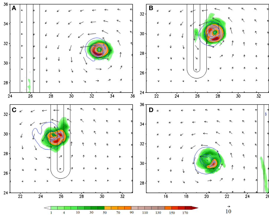
FIGURE 8 | (CNTL/A2) Accumulated 3h rainfall (shaded, in mm/3 h) at (A) 132 h, (B) 168 h, (C) 180 h, and (D) 216 h. The units of the coordinates in the x and y directions are 100 km. The relative vorticity fields are depicted by contours (0.0001, 0.0005, 0.001, 0.002, 0.003 s^{-1} ).
