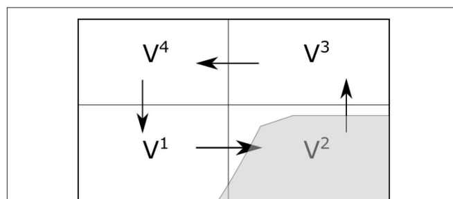
FIGURE 1 | Schematic of the three-dimensional valley-plain system indicating the four control volumes and the mean along-valley circulation during the up-valley wind phase. The arrows indicate the net mass flux across the interfaces between adjacent control volumes. See Figure 3 for a top view of the valley-plain system.
