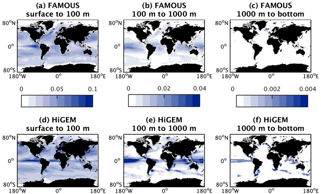
FIG. 2. Global maps of the standard deviation of the temperature tendency [ ^{\circ}\text{C} (12\text{ h})^{-1} ], as calculated from the control runs of (top) FAMOUS and (bottom) HiGEM within the following three depth intervals: (a),(d) from the surface to 100 m (left color bar), (b),(e) from 100 to 1000 m (middle color bar), and (c),(f) from 1000 m to the bottom (right color bar).
