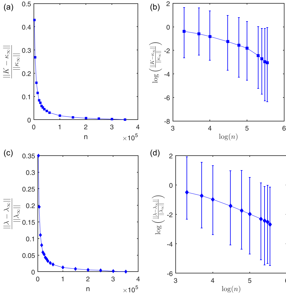
FIG. 1. (a) shows the convergence of the gain minimising the out-of-sample error to the asymptotic gain for increasing n . We plot the quantity \|K - \kappa_\infty\|/\|\kappa_\infty\| against n in blue squares. (b) shows a log plot of the same information with 90% confidence intervals. (c) shows the quantity \|\lambda - \lambda_\infty\|/\|\lambda_\infty\| against n in blue diamonds, where \lambda = (\lambda_1, \lambda_2) represents the eigenvalues of the matrix (A - KHA) . It is evident that the eigenvalues of the matrix (A - KHA) for each gain minimising the out-of-sample error, converge to the eigenvalues of the matrix (A - \kappa_\infty HA) , with n increasing. (d) shows a log plot of the same information with 90% confidence intervals.
