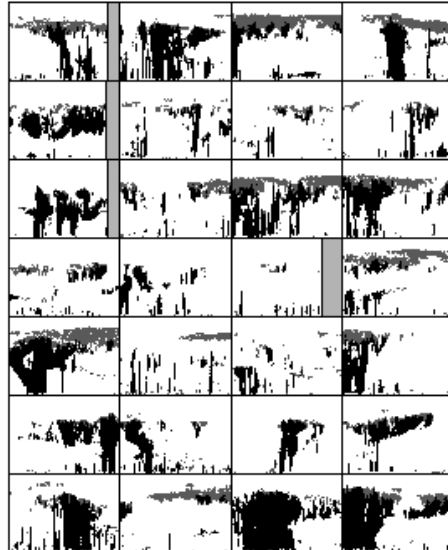
d. Disaggregated, high rainfall SCAI 1–1.25, R 9.5–10.5
