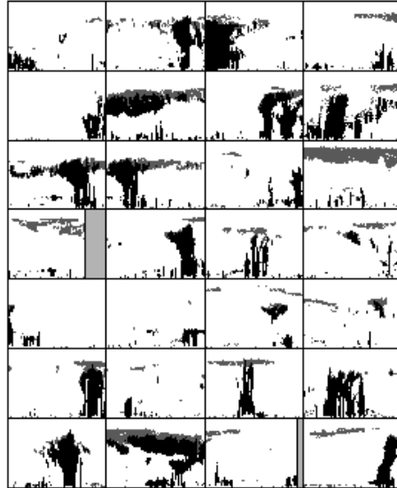
b. Aggregated, high rainfall SCAI 0–0.25, R 9.5–10.5
