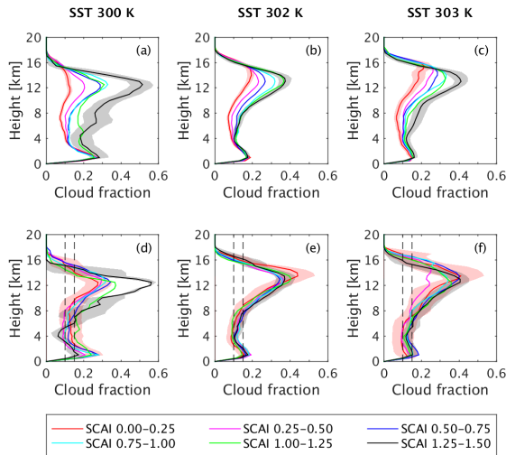
FIG. 11. As in Figure 3, but for rainfall rates between 4.5–5.5 \text{mm day}^{-1} and for SST ranges of (a,d) 299.5–300.5 K, (b,e) 301.5–302.5 K, and (c,f) 302.5–303.5 K.
