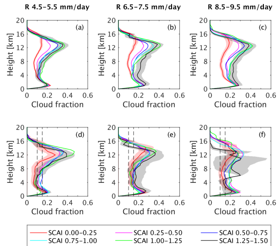
FIG. 3. Average radar-lidar hydrometeor (RLH) fraction for different ranges of SCAI, restricted to rainfall rates of (a) 4.5–5.5 mm day -1 , (b) 6.5–7.5 mm day -1 , and (c) 8.5–9.5 mm day -1 . Different colored lines indicate different SCAI ranges, namely 0–0.25 (red), 0.25–0.50 (magenta), 0.50–0.75 (blue), 0.75–1.00 (cyan), 1.00–1.25 (green), and 1.25–1.50 (black). Shaded areas depict the 90%-confidence intervals for the lowest and highest SCAI ranges. Panels (d)–(f) as in (a)–(c), but restricted to observations with CCA between 0.10 and 0.15 (indicated by the dashed vertical lines).
