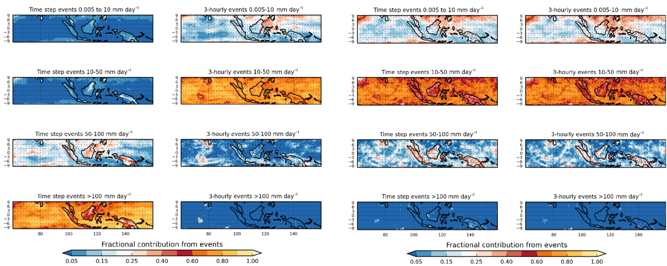
Figure 9. For (a) MetUM-GA3 and (b) ECEarth3, the fractional contributions to the average precipitation rate from ranges of intensity bins shown in the labels above each panel for (left column) time step data and (right column) 3 h means.
