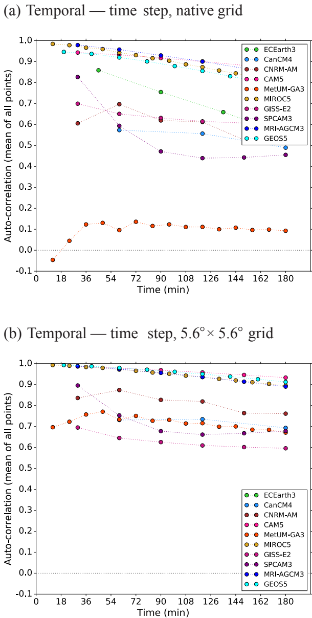
Figure 14. As in Fig. 6b, but for time step rain rates at (a) the native gridscale and (b) averaged to a 5.6^\circ \times 5.6^\circ grid. Panel (a) is repeated from Fig. 6b for ease of comparison.
