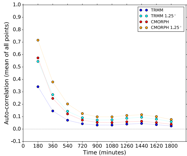
Figure 3. For TRMM 3B42 and CMORPH 0.25° and 1.25° data: (a) a measure of the spatial scale of precipitation features, computed by dividing the analysis domain into 1500\text{ km}\times 1500\text{ km} regions and calculating the lag-0 correlation between the central gridpoint and gridpoints within each distance bin (which are \Delta x wide, starting from 0.5\Delta x ) away from the central gridpoint, then averaging the correlations over all regions in the domain; (b) a measure of the temporal scale of precipitation features, computed as the auto-correlation of precipitation, averaged over all points in the domain. The horizontal lines in (a) show the range of distances spanned by each distance bin; the filled circle is placed at the median distance. For clarity, we omit the correlations for zero distance and zero lag, which are 1.0 by definition.
