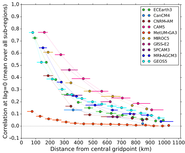
(b) Spatial — 3 h means, native grid
