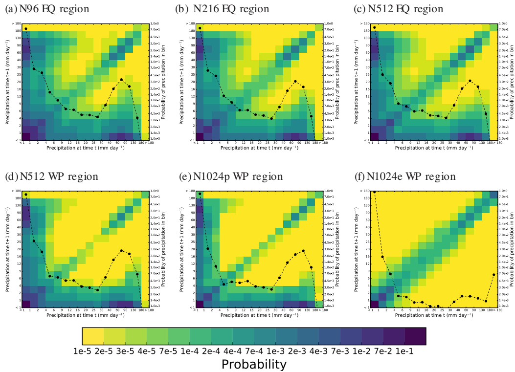
Figure 2. For each MetUM GA6 configuration in Table 1, the filled blocks show the 2-D histogram of binned rain rates (in \text{mm day}^{-1} ) on consecutive time steps at the same grid box, aggregated over all grid boxes; the dashed line shows the 1-D histogram of binned precipitation, using the right-hand vertical axis. Bins were chosen qualitatively such that 3-hourly TRMM analyses over the EQ region have an approximately uniform distribution for rain rates greater than 1 \text{ mm day}^{-1} . Note the logarithmic colour scale.
