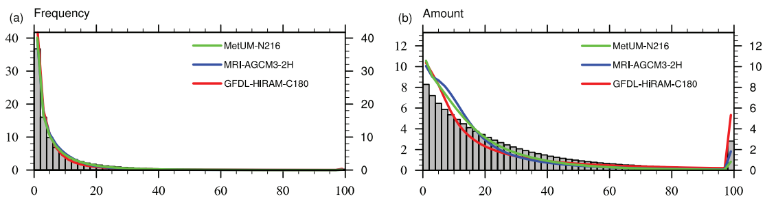
Figure A1. Percentile histograms (bin size 2 \text{ mm day}^{-1} ) of frequency (a) and amount percentile (b) (unit: %) in daily precipitation derived from TRMM and the low resolution models for 1998–2008 covering the globe between 50^\circ\text{S} and 50^\circ\text{N} .
