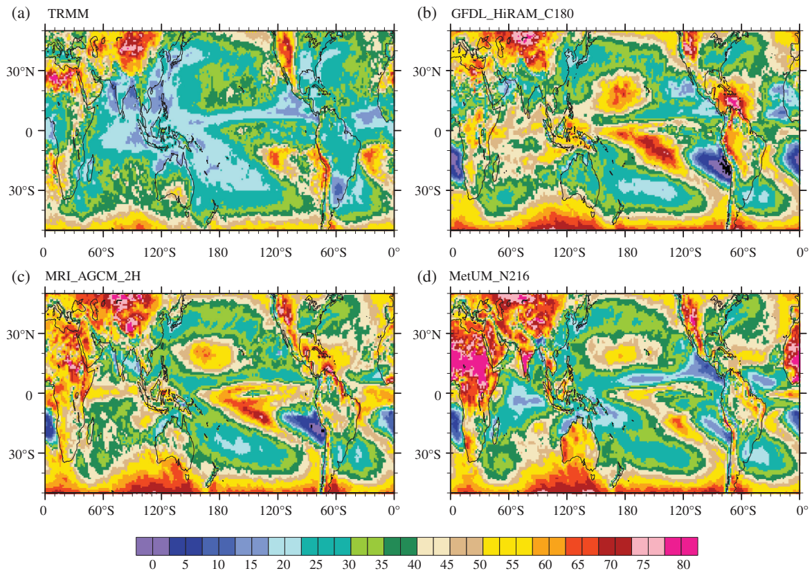
Figure A2. Spatial distribution of amount percentile (unit: %) of light rainfall (bin 1\text{--}11 \text{ mm day}^{-1} ) from (a) TRMM, (b) GFDL-HIRAM-C180, (c) MRI-AGCM-2H and (d) MetUM-N216.
