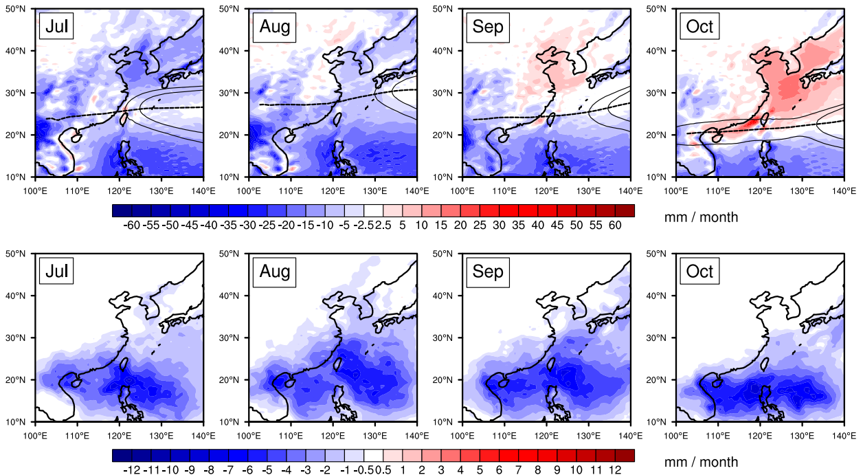
FIG. 4. Monthly accumulated vertically integrated moisture flux divergence for the (top) mean moisture transport [\nabla \cdot (\bar{\mathbf{v}}\bar{q})] and (bottom) TC eddy moisture transport [\nabla \cdot (\bar{\mathbf{v}}q'_{TC} + \mathbf{v}'_{TC}\bar{q} + \mathbf{v}'_{TC}q'_{TC})] (averaged over 1979–2012). Units: \text{mm month}^{-1} . The dashed line in the upper panel indicates the ridge of NWPSH at 500 hPa; Solid lines are geopotential height at 5875 and 5880 m.
