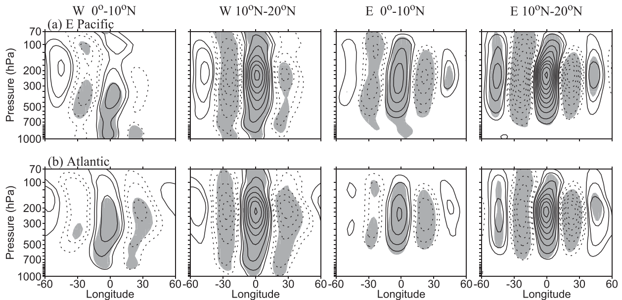
FIG. 11. As in Figs. 1a and 1b, but for waves connected to tropical convection, obtained by regressing v^* in the 0^{\circ} – 10^{\circ} and 10^{\circ} – 20^{\circ} N bands onto the extrema of (left two columns) westward OLR* component and (right two columns) eastward OLR* component at 0^{\circ} – 20^{\circ} N over (a) E. Pacific and (b) Atlantic. The extrema of OLR are located at 0^{\circ} relative longitude with a negative value of 1.5 times its peak standard deviation in the region. Solid (dotted) contours denote positive (negative) winds. Other conventions are as in Fig. 1.
