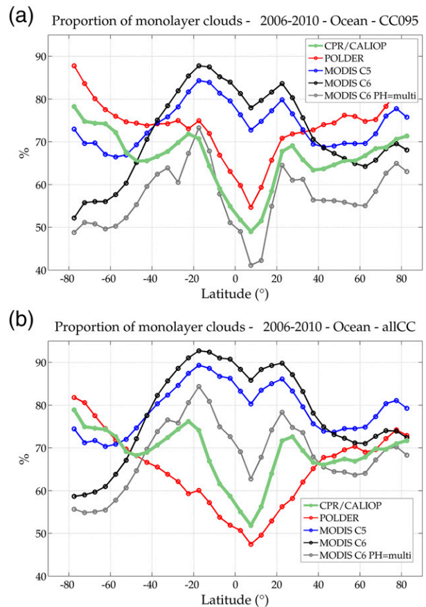
FIG. 10. Zonal proportion of monolayered clouds over 2006–10 from CloudSat /CALIOP, POLDER, and MODIS for (a) clouds over ocean with CC > 0.95 and \tau \geq 5 , and (b) all clouds.
