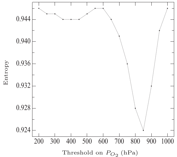
FIG. 3. Entropy of the character monolayer/multilayer conditioned by a threshold on the oxygen pressure P_{\text{O}_2} . The threshold varies between 200 and 1000 hPa in increments of 50 hPa.
