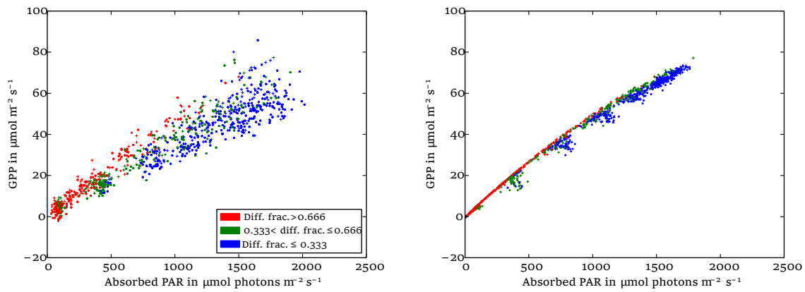
Figure 19. GPP (in \mu\text{mol CO}_2 (\text{m}^2 \text{ground})^{-1} \text{s}^{-1} ) against absorbed PAR (in \mu\text{mol photons } (\text{m}^2 \text{ground})^{-1} \text{s}^{-1} ) for the hourly FLUXNET data (left) and hourly output from the model runs (right). LAI is between 3.5 and 4.5 and all points have DVI less than 1. Dots and vertical crosses (+) indicate US-Ne1 and US-Ne2 respectively. Colour: diffuse radiation fraction. JULES runs have the crop model switched off, LAI and canopy height prescribed and the input parameters in Tables 1, 2, and 4.
