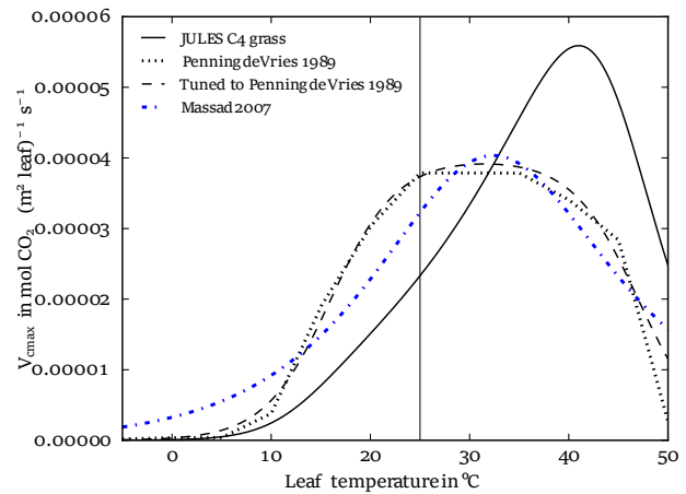
Figure 17. Parametrisations of V_{\text{cmax}} against leaf temperature. Solid black line shows default C4 grass in JULES. Dotted line shows the parametrisation for maize given in de Vries et al. (1989), black dashed line shows a fit to this using the JULES parametrisation. Blue dot-dashed line shows the parametrisation for maize in Massad et al. (2007).
