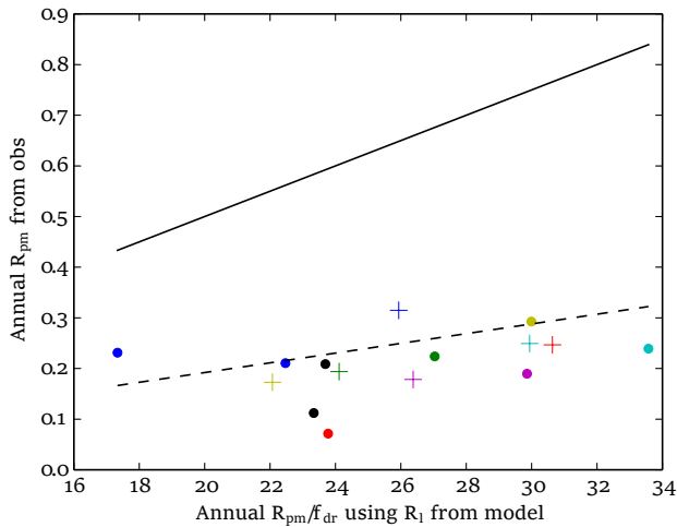
Figure 21. R_{\text{pm}} derived from observed GPP against R_{\text{pm}}/f_{\text{dr}} derived from the outputted model leaf maintenance respiration. Dots and vertical crosses (+) are US-Ne1 and US-Ne2 respectively. JULES runs have the crop model switched off, LAI and canopy height prescribed and the input parameters in Tables 1, 2, 3, and 4. Black lines pass through the origin and have gradient 0.025 (solid line) and 0.0096 (dashed line), corresponding to the value of f_{\text{dr}} used in Osborne et al. (2015) and this study respectively.
