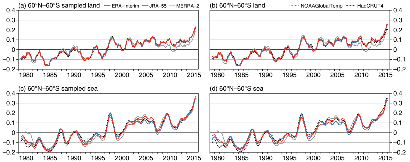
Figure 8. Contributions from (a, b) land and (c, d) sea to 12 month running-mean surface temperature anomalies relative to 1981–2010 (°C) based on data from January 1979 to July 2016, for the region from 60°N to 60°S. (a) and (c) are for HadCRUT4 (black, dotted), ERA-Interim (red, solid), JRA-55 (blue, solid) and MERRA-2 (grey, solid) averaged over the sets of 5° grid boxes where all datasets provide values for land and sea respectively. (b) and (d) are for HadCRUT4 and NOAA GlobalTemp averaged over all grid boxes where each separately provides values, and for ERA-Interim, JRA-55 and MERRA-2 averaged over all land and sea.
