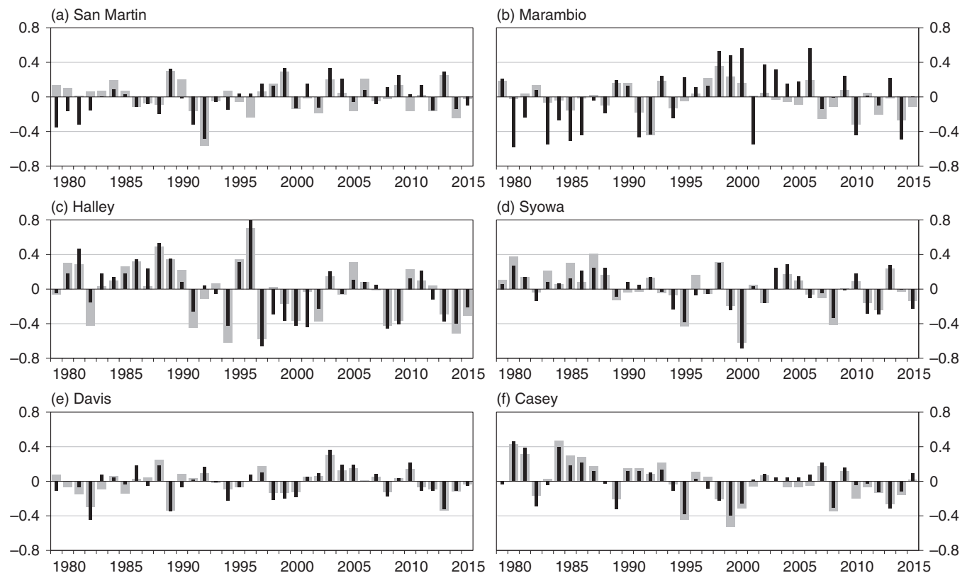
Figure 7. Annual-mean surface air temperature anomalies (°C) relative to 1981–2010, at (a) San Martin (68.1°S, 67.1°W), (b) Marambio (64.2°S, 56.7°W) (c) Halley (75.6°S, 26.7°W), (d) Syowa (69.0°S, 39.6°E), (e) Davis (68.6°S, 78.0°E) and (f) Casey (66.3°S, 110.5°E). Narrow, darker bars denote observed station values and broader, lighter bars denote corresponding ERA-Interim background forecast values.
