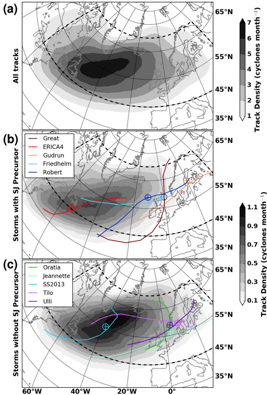
FIG. 4. Extratropical cyclone track density, defined as number density per month in a unit area equivalent to a 5° spherical cap (approximately 10 6 km 2 ) with cyclones counted only once per spherical cap, for cyclones occurring during September–May seasons through 1979–2012 with vorticity maxima within the dashed black curve. (a) Track density for all cyclones. Track density for explosively developing ( \Delta\text{MSLP}_{\text{min}} < -20 hPa over 24 h) cyclones (b) without and (c) with sting-jet precursors; selected tracks (based on \zeta_{850} with locations of lowest MSLP marked by circles with plus sign) from cyclones with published case studies are shown by colored lines with legend.
