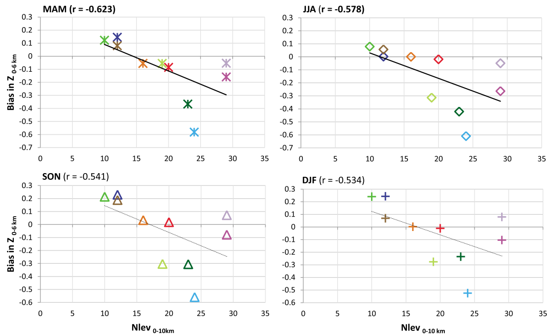
AeroCom II Models: GOCART, SPRINTARS, LSCE, GMI-MERRA-v3, ECHAM-HAM, PNNL, GISS-MATRIX, Oslo-CTM2, HadGEM, CAM4_Oslo
