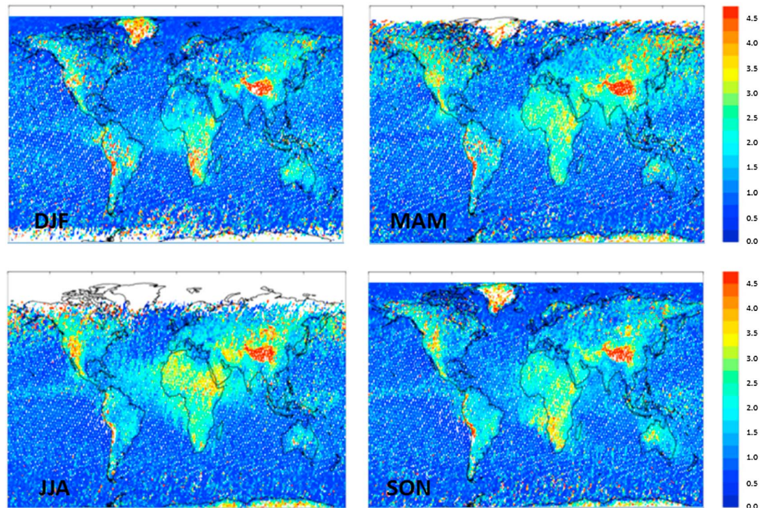
Figure 1. Illustration of the AeroCom-CALIOP 3-D global 1^\circ \times 1^\circ gridded product: 2009 Z_{\alpha 0-6 \text{ km}} mean seasonal aerosol extinction height (km) over the 0–6 km altitude range.
