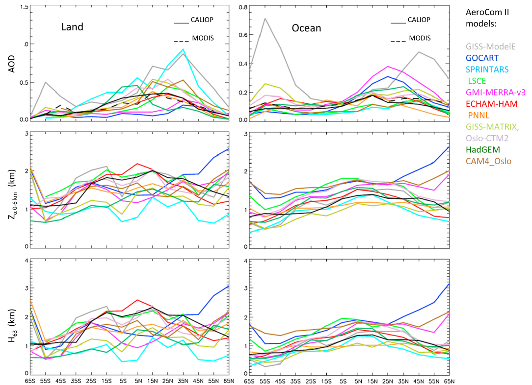
Figure 9. Models (2006) and CALIOP (2007–2009) mean annual latitudinal gradient of the (first row) AOD, (second row) Z_{\alpha-0-6 \text{ km}} , and (third row) H_{63} aerosol diagnostics over the 0–6 km altitude range (14 latitude bands), over (left column) land and (right column) ocean. MODIS AOD is also reported.
