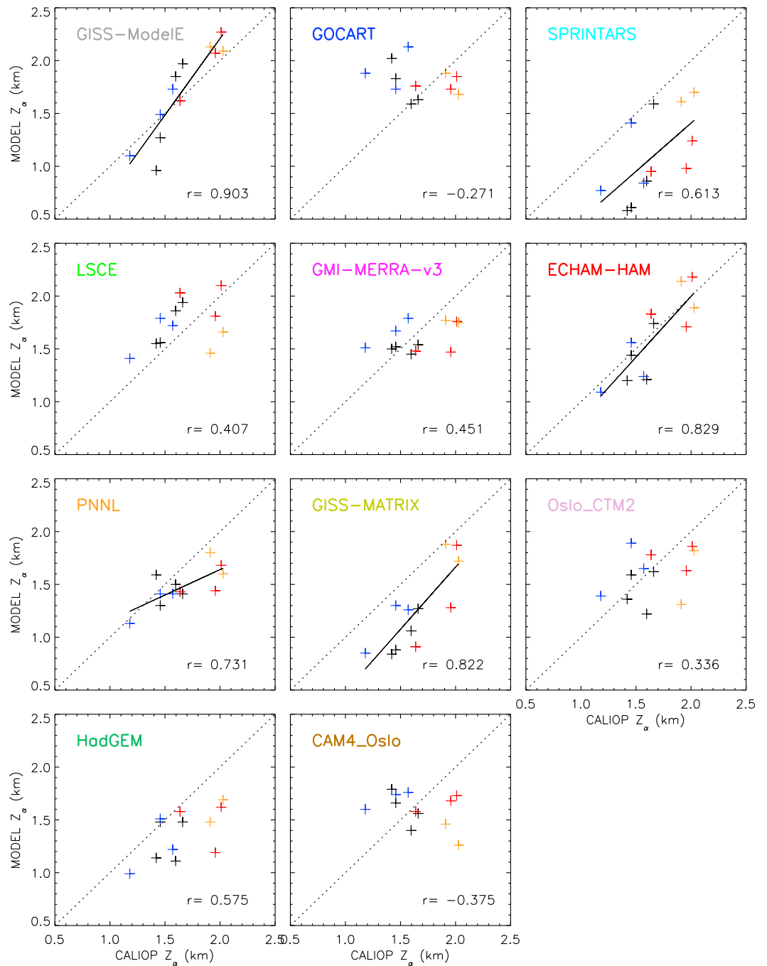
Figure 6. Models (2006) versus CALIOP (2007–2009) mean annual Z_{\alpha 0-6} km aerosol extinction height over the 12 selected regions (see Figure 2 for the definition of the domains and the color legend). Significant ( p < 0.05 ) regression lines are plotted.
