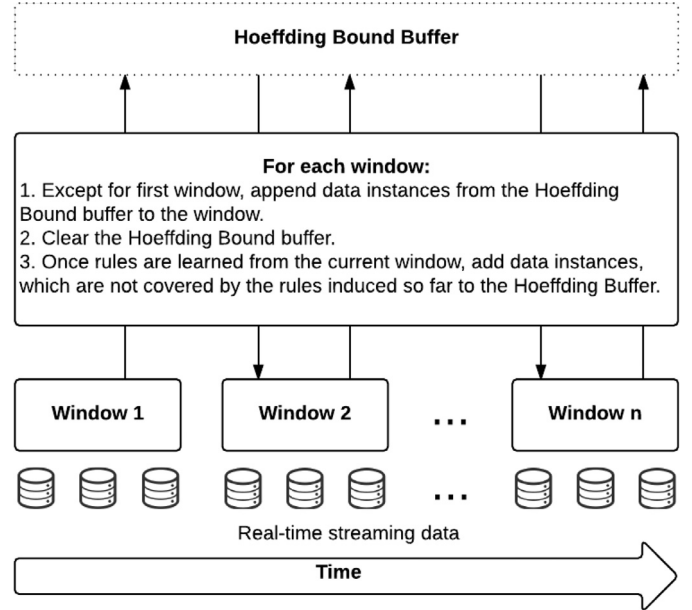
Fig. 6. Combining data instances that satisfy the Hoeffding bound from the previous window with the unseen data instances from the current window.
