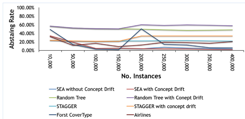
Fig. 10. Abstaining rates of Hoefding Rules.
