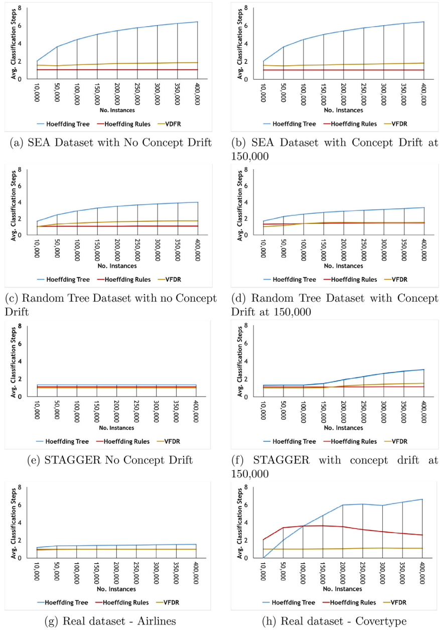
Fig. 9. The average number of classification steps needed by Hoefding Rules compared with Hoefding Tree and VFDR.
