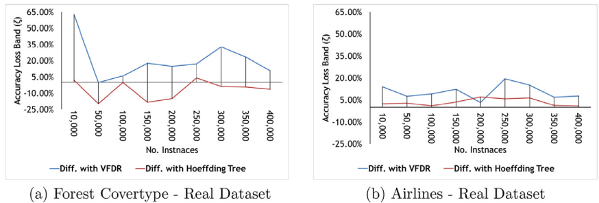
Fig. 8. Difference in accuracy compared with other classifiers for real data streams.
