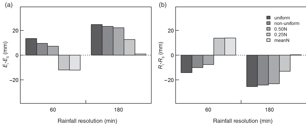
Figure 8. Annual difference in (a) evaporation E and (b) runoff R for 60- and 180-min precipitation forcing data (subscript i ) downscaled to 5-min (subscript 5) using various disaggregation methods (legend) for Swindon 2012.
