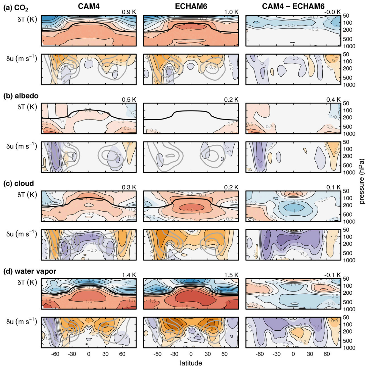
FIG. 2. Zonal-mean temperature and zonal wind responses to (a) CO 2 doubling with no feedbacks and (b)–(d) imposed albedo, cloud, and water vapor feedbacks, respectively. The total response (sum of CO 2 forcing and imposed feedbacks) is shown in Fig. 1, center. Thick gray contours indicate the zonal wind climatology (only positive values shown; contour interval 10 m s^{-1} ). The black curves in the temperature plots denote the tropopause height. Changes in global-mean surface temperature are indicated at the top-right corner of each temperature plot.
