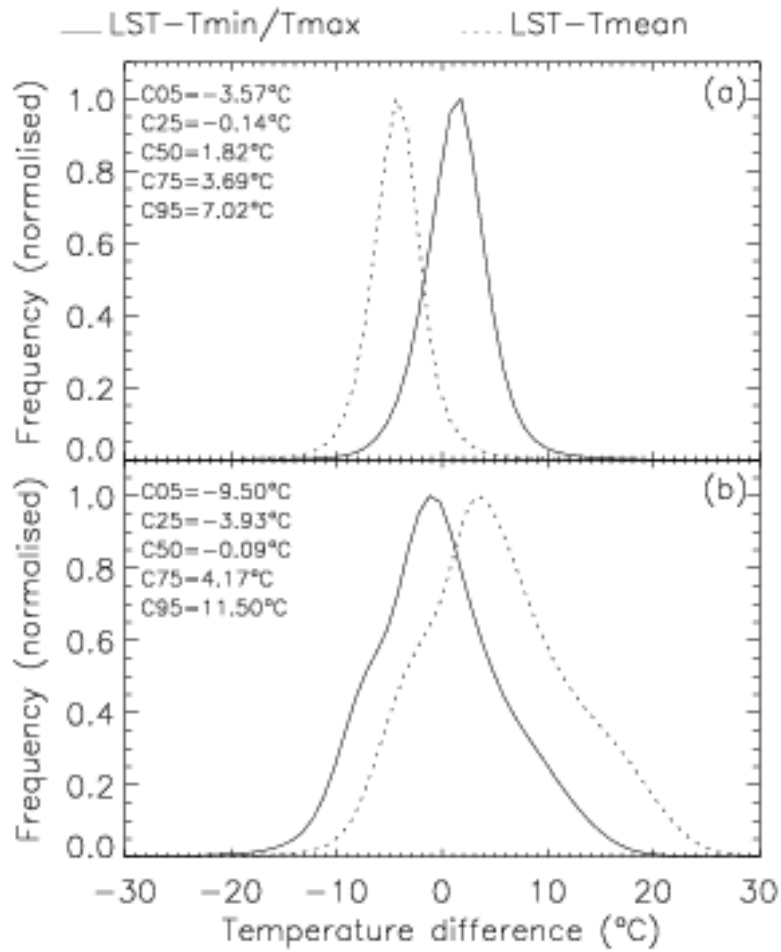
Figure 6: Normalised distributions of the CDR minus CRU TS differences for (a) LST_{\text{night}} - T_{\text{min}} (solid line) and LST_{\text{night}} - T_{\text{mean}} (dotted line) and (b) LST_{\text{day}} - T_{\text{max}} (solid line) and LST_{\text{day}} - T_{\text{mean}} (dotted line). The histograms are calculated from data acquired August 1995 through March 2012. The 5 th (C05), 25 th (C25), 50 th (C50), 75 th (C75) and 95 th (C95) centiles of the LST_{\text{night}} - T_{\text{min}} (a) and LST_{\text{day}} - T_{\text{max}} (b) differences are shown on each panel.
