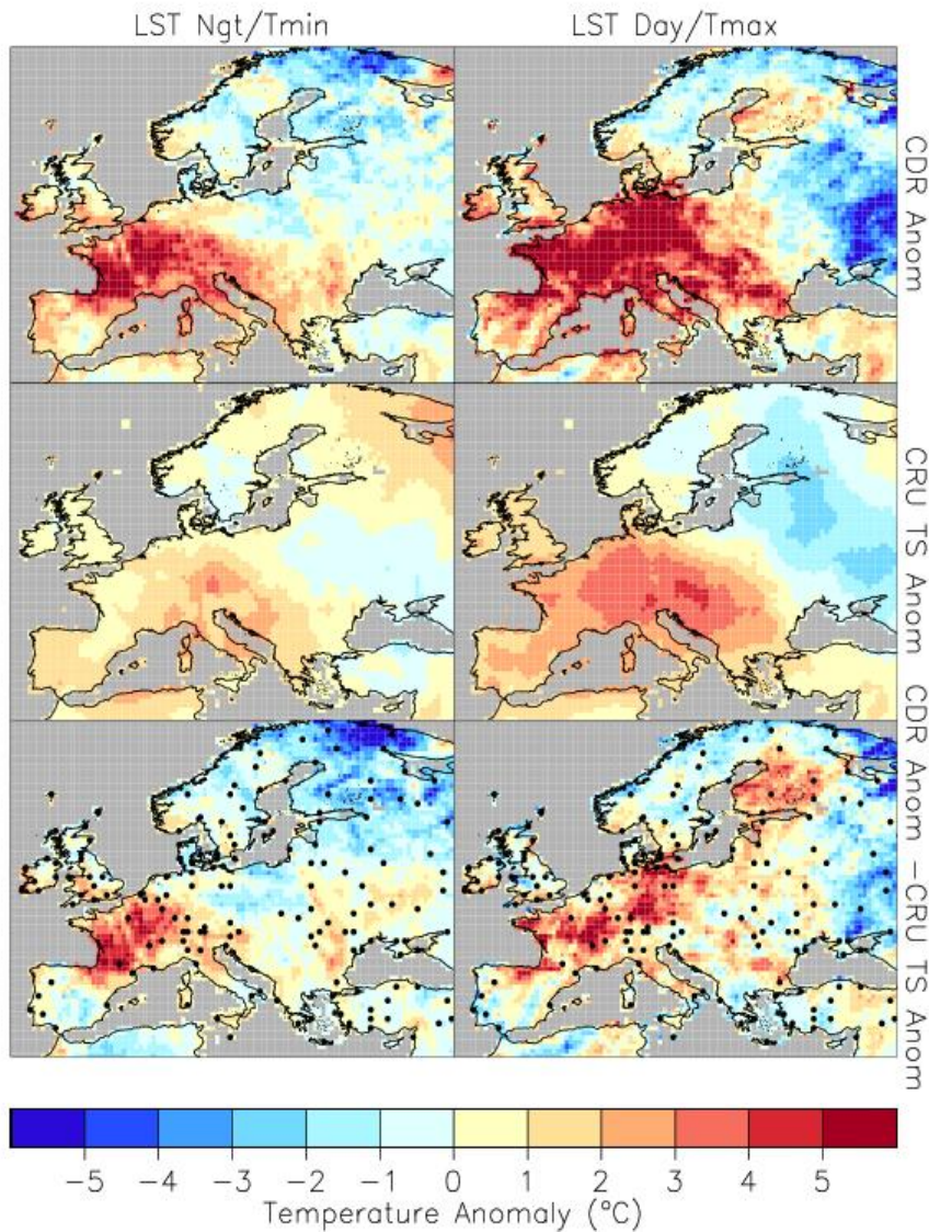
Figure 16: Temperature anomalies ( ^{\circ}\text{C} ) for the August 2003 European heat wave for LST night/ T_{\text{min}} (left) and LST day/ T_{\text{max}} (right). Both the CDR (top) and CRU TS (middle) anomalies are referenced to the August 1995-March 2012 baseline period – both are shown at a spatial resolution of 0.5^{\circ} . The bottom row shows the difference between the two, with the location of the CRU TS stations overlaid (filled black circles).
