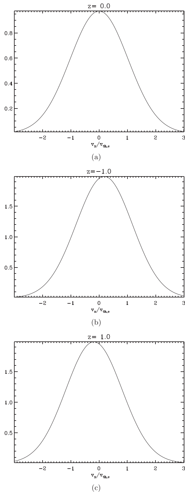
FIG. 1. The v_x variation of f_e for z/L = 0 (a), z/L = -1 (b), and z/L = 1 (c). \beta_{pl} = 0.85 and \delta_e = 0.15 . Note the antisymmetry of the z = \pm 1 plots with respect to each other.
