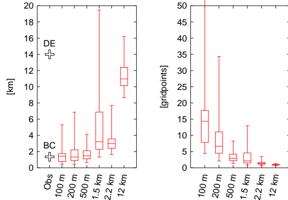
Figure 8: Frontal widths, calculated as described in the text, in units of (a) km and (b) gridpoints. The box-and-whisker symbols indicate the median, interquartile range and full range from the sample of circuits. The crosses in (a) are the observed values from the two transects, as indicated.
