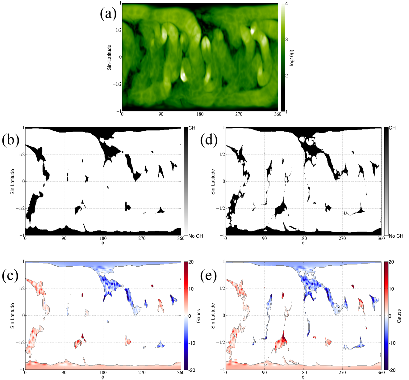
Fig. 4.— (a) Simulated AIA 193Å map from the thermodynamic MHD model using the NSO VSM CR2098 map for the boundary condition. This map is used to test the CH detection method. (b) The CHs (black regions) identified when the CH detection method is applied to the simulated data. (c) The magnetic field in the CH, obtained by overlaying (b) with the NSO VSM map (as was done in Figure 3). (d) The true open field regions for the model. (e) The true open magnetic field in the model.
