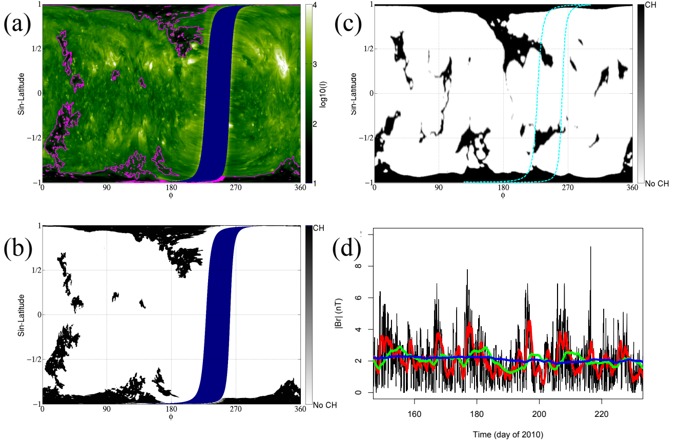
Fig. 1.— (a) Synchronic EUV map for July 8, 2010 at 18:00, compiled from STEREO A & B EUVI 195Å and SDO AIA 193Å images. The magenta lines show the coronal hole detections. The sector near 270°, indicated by the blue swath, was not observed. (b) The detected coronal holes (black regions) from (a). (c) Open field regions (black) from a thermodynamic MHD model with boundary derived from an ADAPT map. The unobserved region is indicated with cyan dashed lines. (d) OMNI in situ measurements of B_r for 80 days surrounding the time period of interest. A 1-hour running average of |B_r| (black line), 1-day running average (red), 7-day (green) and Carrington rotation average (blue) are shown.
