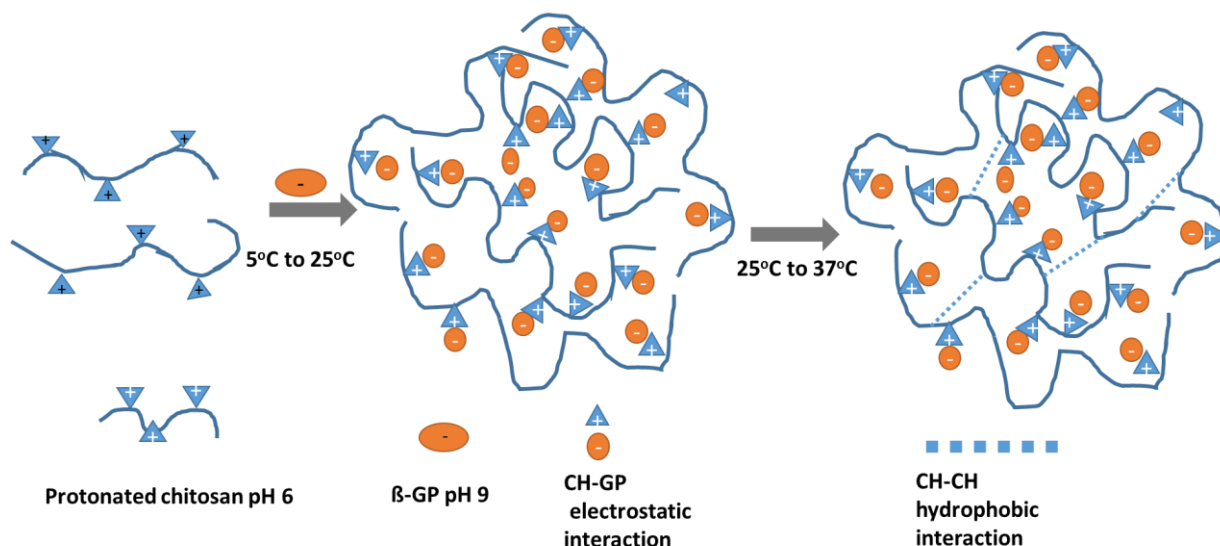
Figure 5: Schematic diagram showing gelation process of chitosan/β-glycerophosphate mixture at 37°C
