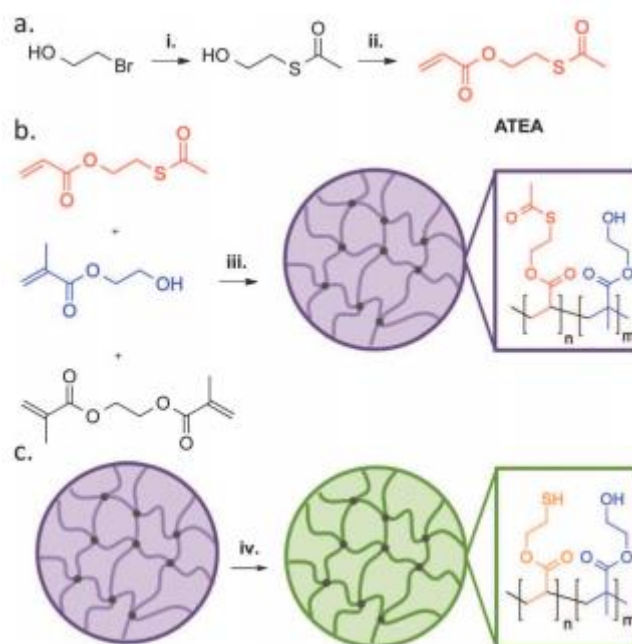
Figure 4: Synthesis of thiolated microgels: (a) Synthetic route to ATEA, a protected thiomonomer. (b) Polymerisation to form ATEA: HEMA copolymer microgels, displaying the pendant functionalities present. (c) Deprotection of ATEA using sodium thiomethoxide to yield thiol-bearing microgels. (i) Potassium thioacetate, acetone, 24 h. (ii) Acryloyl chloride, trimethylamine, DCM, reflux, 24 h. (iii) Ammonium persulfate, ethylene glycol dimethacrylate, water, 70°C, 6 h. (iv) Sodium thiomethoxide, methanol, 30 min. This figure is reproduced from Cook et al., (2015). Reproduced with permission from the Royal Society of Chemistry.
