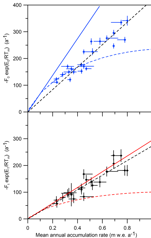
Figure 13. (top) -F_0 \exp(E_0/RT_m) and (bottom) -F_t \exp(E_1/RT_m) as a function of mean annual accumulation rate. The activation energies are set to the Arthern value E_0 = E_1 = 17.6 \text{ kJ mol}^{-1} . The blue and red solid lines show the curves expected for stages 1 and 2 from the Arthern model and the blue and red dashed lines the curves expected from the Ligtenberg model. Black dashed lines show the best fit to the data through the origin.
