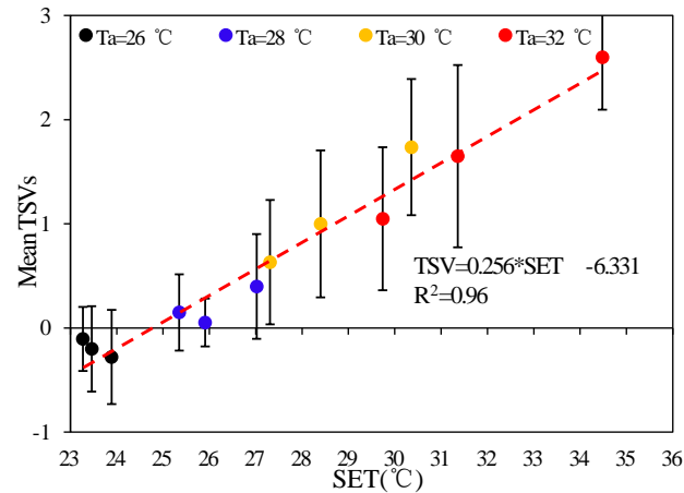
Figure 5: The relationship between SET and TSV under different relative humidity conditions
