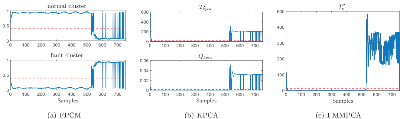
Fig. 8. Monitoring charts of Fault 4
