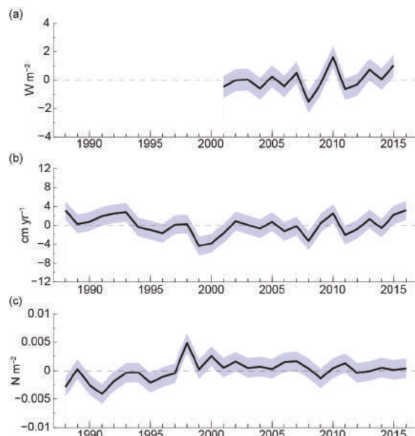
FIG. 3.14. Annual-mean time series of global averages of (a) net surface heat flux ( Q_{\text{net}} ; \text{W m}^{-2} ) from the combination of CERES EBAF SW+LW and OAFIux-HR LH+SH, (b) net freshwater flux ( P-E ; \text{cm yr}^{-1} ) from the combination of GPCP P and OAFIux-HR E , and (c) wind stress magnitude ( \text{N m}^{-2} ) from OAFIux-HR vector wind analysis. Shaded area denotes one std. dev. of annual-mean variability.
