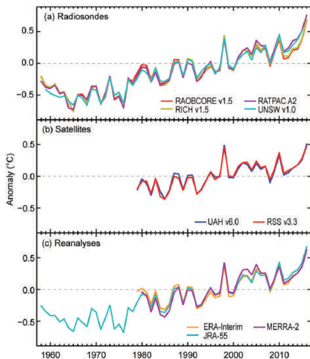
FIG. 2.6. Global average lower tropospheric temperature annual anomalies (°C; 1981–2010 base period for the MSU LT equivalent layer). (a) Radiosonde: RATPAC (Free et al. 2005), RAOBCORE and RICH (Haimberger et al. 2012) and UNSW (Sherwood and Nishant 2015). (b) Satellites: UAHv6.0 (Spencer et al. 2017) and RSSv3.3 (Mears and Wentz 2009). (c) Reanalyses: ERA-Interim (Dee et al. 2011), MERRA-2 (Bosilovich et al. 2015; Gelaro et al. 2017), and JRA-55 (Ebita et al. 2011; Kobayashi et al. 2015).
