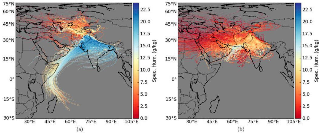
FIG. 12. The 6-day back trajectories for each of the 100 strongest relative EPEs for (a) June–September and (b) December–April. For each event, we take a cuboid of 300 km on a side between 925 and 500 hPa during the day of the EPE, finding the 10 voxels therein with the highest relative humidity. These are backtracked, giving 1000 trajectories in total.
