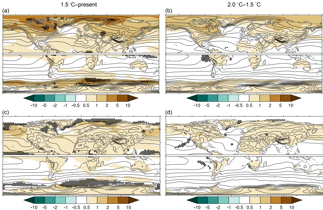
Figure 1. Multi-model mean response of surface air temperature for 1.5°C–PD ( a, c ) and 2.0–1.5°C ( b, d ). Panels ( a ) and ( b ) show winter (Northern Hemisphere DJF, Southern Hemisphere JJA) responses (shading; units K) along with the climatology (contour interval 5 K) for the ( a ) PD and ( b ) 1.5°C experiments. Panels ( c ) and ( d ) show the same for summer (Northern Hemisphere JJA, Southern Hemisphere DJF) along with the climatology (contour interval 5 K) for the ( c ) PD and ( d ) 1.5°C experiments. There is model consensus on the sign of the response everywhere. Black dots mask out regions where there is model dependence; i.e. the models do not agree on the magnitude of the response ( f^2 > 1 ; see Sect. 2.2 for details).
