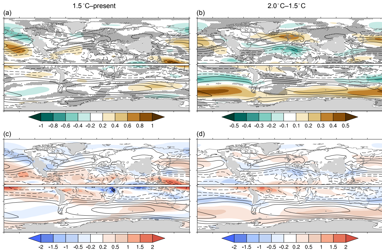
Figure 4. Multi-model mean response of winter (Northern Hemisphere DJF, Southern Hemisphere JJA) zonal wind at 850 hPa ( u_{850} ) for 1.5°C–PD ( a , c ) and 2.0–1.5°C ( b , d ). Panels ( a ) and ( b ) show responses (shading; units \text{m s}^{-1} ) along with the climatology (contour interval 4 \text{ m s}^{-1} ) for the ( a ) PD and ( b ) 1.5°C experiments. Note the different colour scale for ( a ) and ( b ). Panels ( c ) and ( d ) show signal-to-noise ratio \beta/\sigma , where the sign corresponds to the sign of the response, along with the climatology (contour interval 4 \text{ m s}^{-1} ) for the ( c ) 1.5°C and ( d ) 2.0°C experiments. In ( a ) and ( b ), hatching masks out regions where there is no model consensus (fewer than four out of five models agree) on the sign of the response. In ( c ) and ( d ), black dots mask out regions where the models do not agree on the magnitude of the response ( f^2 > 1 ). Grey shading indicates regions of high topography intersecting the plotted variable.
