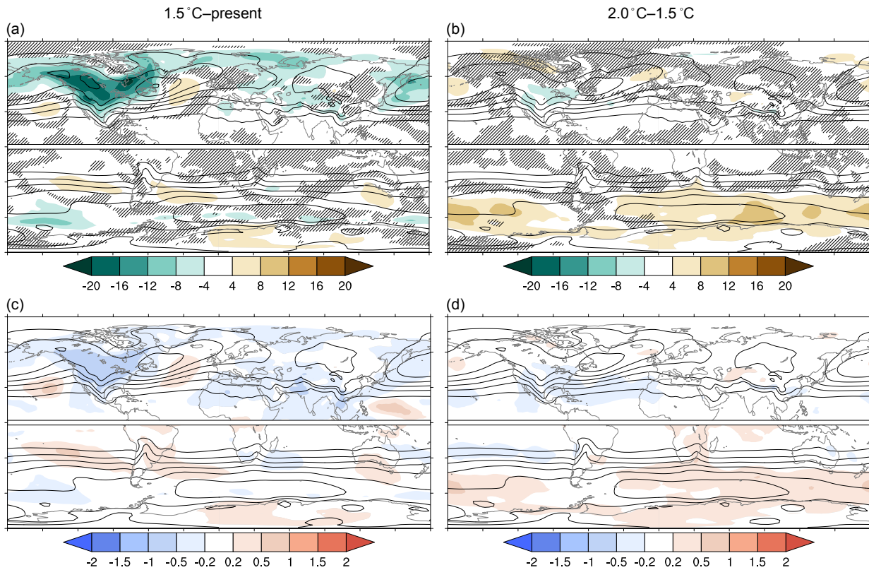
Figure 8. Multi-model mean response of winter (Northern Hemisphere DJF, Southern Hemisphere JJA) low-level MSLP' storm tracks for 1.5°C-PD (a, c) and 2.0–1.5°C (b, d). Panels (a) and (b) show responses (shading; units hPa) along with the climatology (contour interval 100 hPa) for the (a) PD and (b) 1.5°C experiments. Panels (c) and (d) show signal-to-noise ratio \beta/\sigma , where the sign corresponds to the sign of the response, along with the climatology (contour interval 100 hPa) for the (c) 1.5°C and (d) 2.0°C experiments. In (a) and (b), hatching masks out regions where there is no model consensus (fewer than four out of five models agree) on the sign of the response. In (c) and (d), black dots mask out regions where the models do not agree on the magnitude of the response ( f^2 > 1 ). The storm tracks are defined as the standard deviation of bandpass filtered daily MSLP.
