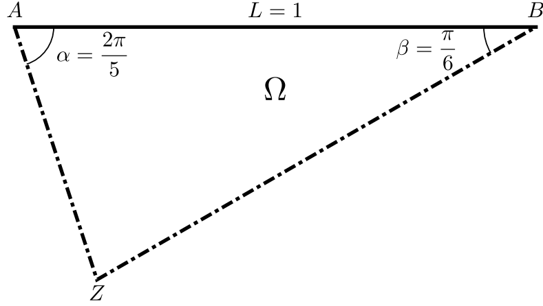
Figure 5: Triangle from Example C.1
