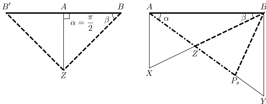
Figure 4: Construction of auxiliary triangles in the case \alpha = \pi/2 (left) and \alpha < \pi/2 (right)
