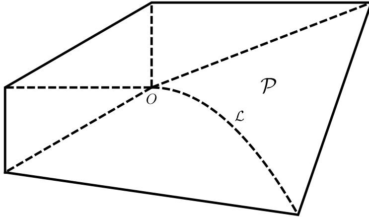
Figure 3: A polygon with auxiliary curves \mathcal{L}
