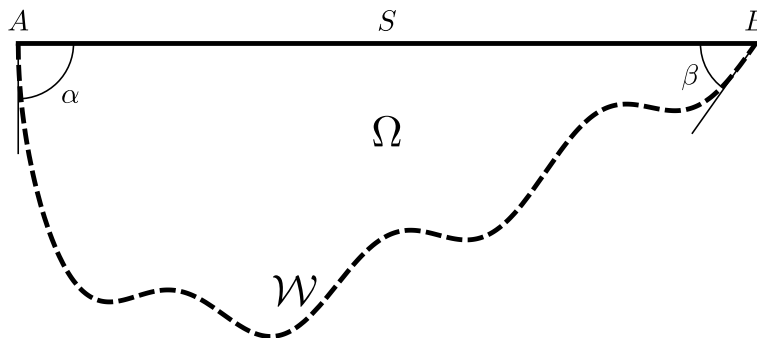
Figure 1: Geometry of the sloshing problem
