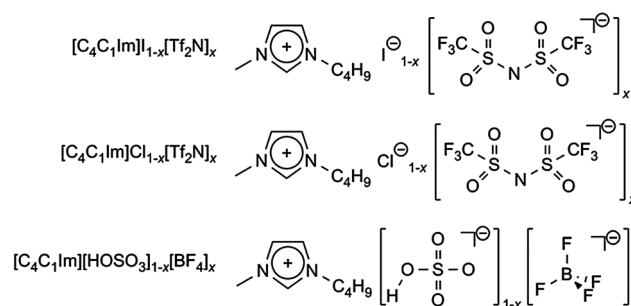
Scheme 1 Three ionic liquid mixture systems investigated in this communication.
