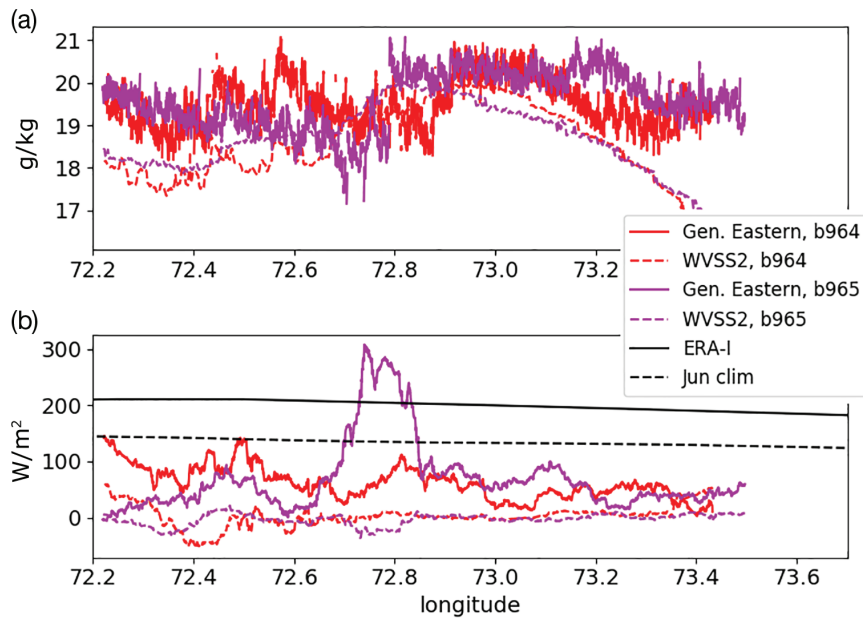
FIGURE 13 (a) Specific humidity (g/kg) and (b) estimates of surface latent heat flux ( W/m^2 ) from low-level runs over the Arabian Sea (colours), ERA-Interim on 26 June, 0000–1200 UTC mean (solid black, 0530 to 1730 local time), and Goddard Satellite-based Surface Turbulent Fluxes (GSSTF, dashed black) climatology for June 1998–2008 [Colour figure can be viewed at wileyonlinelibrary.com ]
