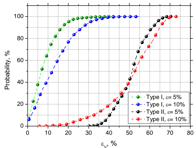
Figure 10. Cumulative probability of the uncertainty \varepsilon_v in the volume concentration retrieval from the PFR data set with input errors \varepsilon = 5\% and 10\% for Type I and Type II PSDs.
