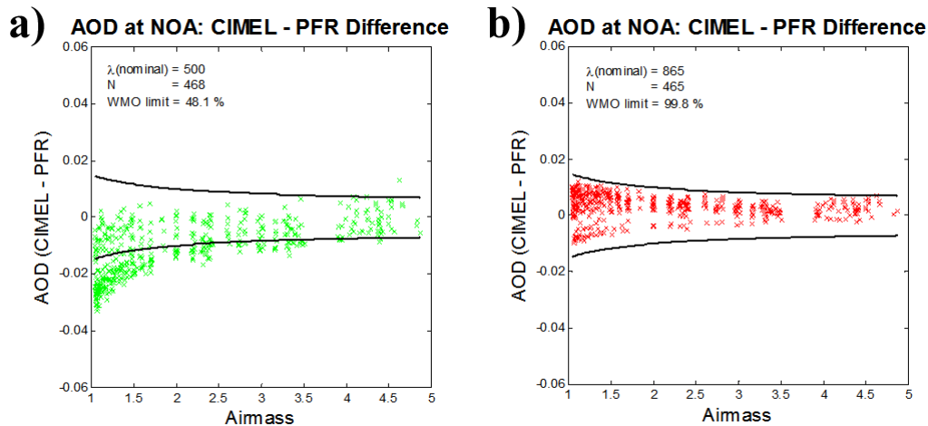
Figure 4. AOD difference (CIMEL-PFR) versus air mass at NOA illustrating the WMO criteria for traceability (solid line) at (a) 500 nm (green) and (b) 865 nm (red).
