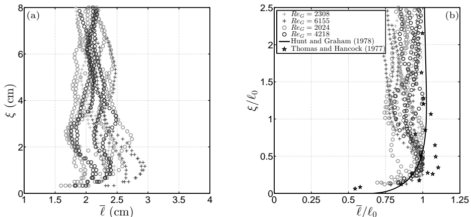
FIGURE 5. (a) Computed values of the time-averaged integral length scale, \bar{l} , plotted against height \xi . (b) The same data but scaled by the reference integral length scale, \ell_0 , from each experiment. The data obtained using the coarse and fine grids are shown separately, indicated by the circles and crosses, respectively. The data shown are from the representative subset of experiments (indicated by the † superscripts in table 1) for Re_G = 2024, 2308, 4218 and 6155 [see legend in (b)]. For each Re_G , data from the n repeats are shown, where n = 2, 4 or 5 (see table 1). Also shown in (b) are corresponding experimental data from Thomas & Hancock (1977) and a prediction based on RDT by Hunt & Graham (1978) (see legend).
