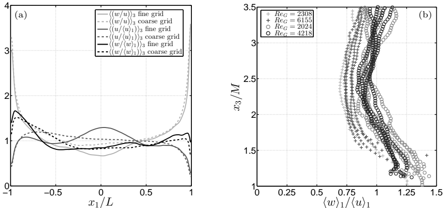
FIGURE 2. (a) Normalised profiles \langle u/\langle u \rangle_3 \rangle_3 , \langle w/\langle w \rangle_3 \rangle_3 (homogeneity) and the isotropy parameter \langle w/\langle w \rangle_3 \rangle_3 , each spatially averaged in x_3 and plotted against the horizontal x_1 coordinate, which has been scaled by the half-width of the inner box, L . Data obtained using the fine and coarse grids are shown separately (see legend). (b) Measurements of the isotropy parameter \langle w \rangle_1 / \langle u \rangle_1 plotted against x_3/M (which, recall, have been spatially averaged across the central 50% of the inner box's width). The data shown are from the representative subset of experiments (indicated by the † superscripts in table 1) for Re_G = 2024, 2308, 4218 and 6155 (see legend). For each Re_G , data from the n repeats are shown, where n = 2, 4 or 5 (see table 1). The data obtained using the coarse and fine grids are shown separately, indicated by the circles and crosses respectively.
