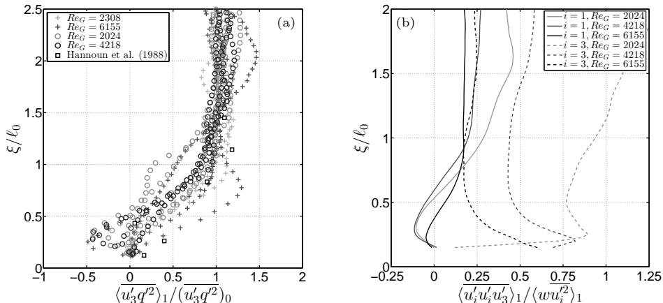
FIGURE 9. (a) Measurements of the vertical flux of TKE, \langle \overline{u'_3 q'^2} \rangle_1 , plotted against scaled height \xi / \ell_0 . The data have been normalised by the trend expected in the absence of the floor plate, denoted \langle \overline{u'_3 q'^2} \rangle_0 . The data shown are from the representative subset of experiments (indicated by the † superscripts in table 1) for Re_G = 2024, 2308, 4218 and 6155 (see legend). For each Re_G , data from the n repeats are shown, where n = 2, 4 or 5 (see table 1). Also shown are data taken from Hannoun et al. (1988). (b) Measurements of correlation coefficients \langle \overline{u'_i u'_i u'_3} \rangle_1 / \langle \overline{w u_i'^2} \rangle_1 for i = 1 and i = 3 (with the summation convention dropped), plotted against scaled height \xi / \ell_0 . The data are shown are from the representative subset of experiments, for Re_G = 2024, 4218 and 6155 (see legend).
