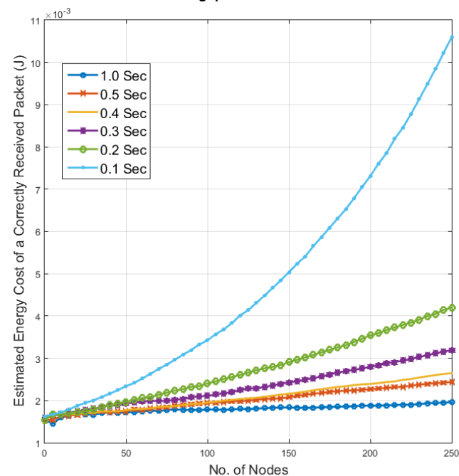
FIGURE 9. Energy (J) cost of a correctly received packet with varied advInterval .
