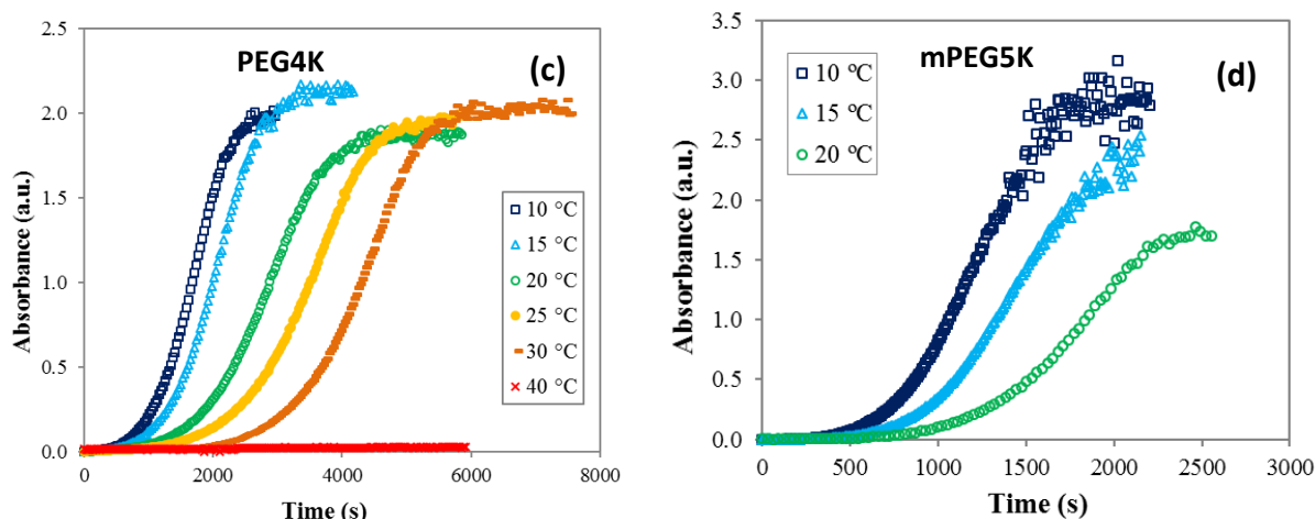
Figure 2. UV-Vis absorbance monitoring the complexation process as a function of temperature in four PEG systems at a constant concentration of 5% \alpha -CD: (a) 0.55% SiPEG5K#3 (equivalent 0.3% PEG); (b) 0.33% mPEGMa5K; (c) 0.3% PEG4K; and (d) 0.33% mPEG5K.
