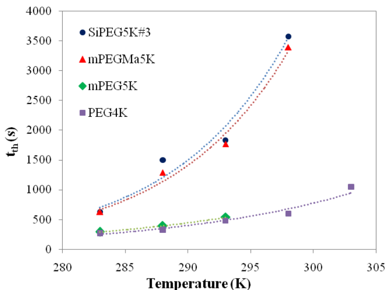
Figure 3. Reaction times at “threading” for the curves obtained from the UV-vis analysis of the complexation between \alpha -CD and the PEG samples studied as a function of temperature (threading times t_{th} were considered when absorbances reached a value of 0.01).
