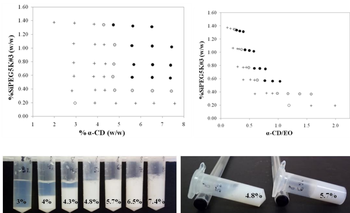
Figure 8. Phase diagram for mixtures of SiPEG5K#3 nanoparticles and \alpha -CD in aqueous solution: ( \circ ) solution, (+) biphasic system, ( \bullet ) weak gel, ( \bullet ) gel shown in two representations: as a function of \alpha -CD wt.% (top left) and \alpha -CD/EO molar ratio (top right). Bottom: Pictures showing the appearance of complexes of SiPEG5K#3 (0.8% w/w) with \alpha -CD up to 7.4% w/w after 7 days (left); samples with 4.8% (weak gel) and 5.7% (gel) \alpha -CD after 7 days (right).
