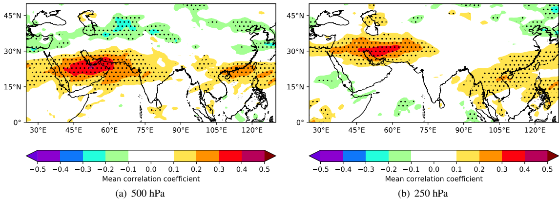
FIG. 4. Interannual correlation coefficients between the monthly mean baroclinic angle at (a) 500 hPa and (b) 250 hPa and the monthly western disturbance frequency, computed using ERA-Interim, December - March. The reanalysis data were coarsened to match the available vertical resolution from the CMIP5 output, so that calculations based on vertical gradients were consistent. Stippling indicates where the correlation coefficient was significant at the 90% confidence level. Note that the colour scales differ between here and Fig. 5.
