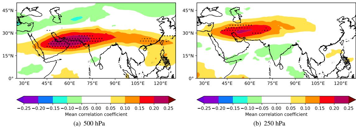
FIG. 5. As Fig. 4 but showing the multi-model mean of correlations computed for each CMIP5 model. Stippling indicates where at least half of the models had a correlation coefficient that was significant at the 90% confidence level. Computed for December - March.
