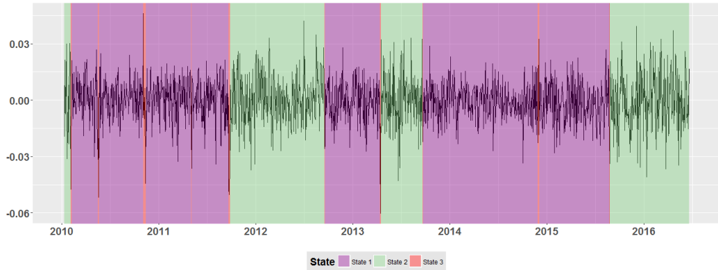
Figure 19: Global Decoding of Fitted three-state HSMM for Platinum
