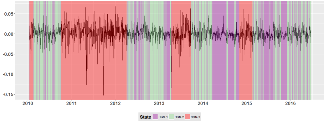
Figure 18: Global Decoding of Fitted three-state HSMM for Silver
