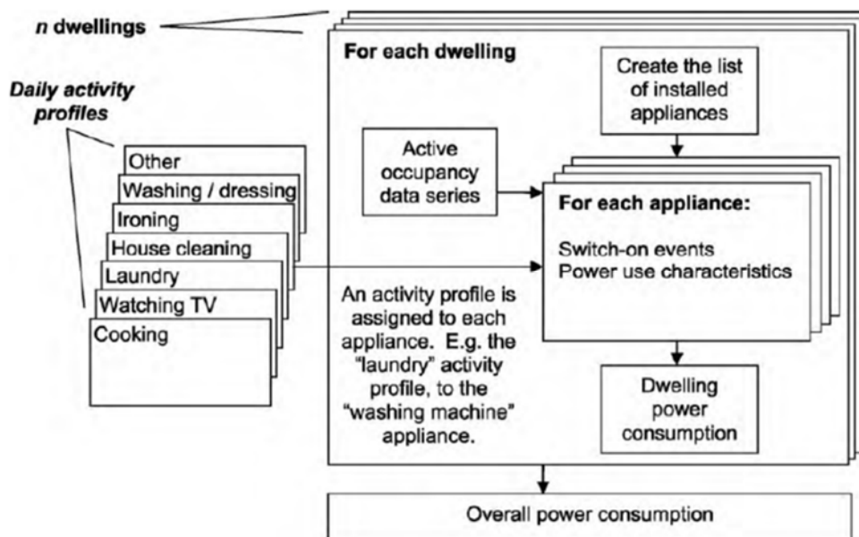
Figure 4: Electricity demand model architecture (Source: Richardson et al. 2010)
