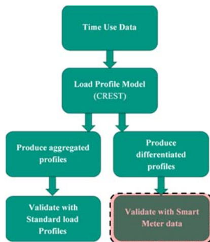
Figure 2: Visual presentation of the overall approach
