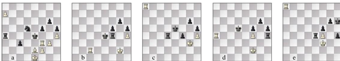
Fig. 3. Navrotescu-Shah: as played (a) 56w and (b) 65w, hypothetically leading with SF ± to (c) 103w after f4; the easier win (d) 66w after Rxa4 leading with SF ± to (e) 75w after h4.
