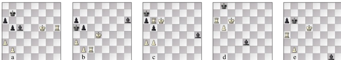
Fig. 5. Tiviakov–Korsunsky: positions in the played line, (a) 45w, (b) 62w, (c) 71b and (d) 79b. The SF ± FINALGEN line chosen converts to KRPKBP at (e) position 51b.
