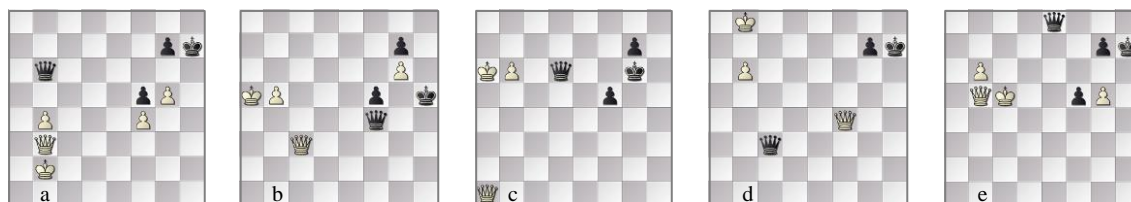
Fig. 6. LC0-Et: (a) 94w; FINALGEN-optimal line (b) 105w before b6"", (c) 7m 116w and (d) 6m 128b; (e) drawn 175b.
