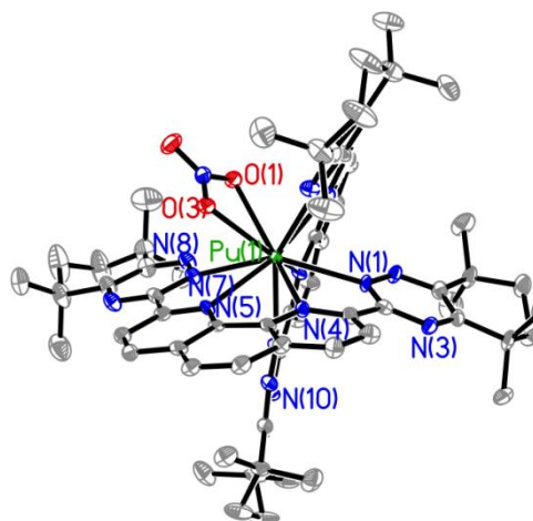
Figure 2. Thermal ellipsoid plot of the solid-state structure of [\text{Pu}^{\text{III}}(\text{CyMe}_4\text{-BTPPhen})_2(\text{NO}_3)]_2[\text{Pu}^{\text{IV}}(\text{NO}_3)_6] \cdot 4\text{MeCN} . The [\text{Pu}^{\text{IV}}(\text{NO}_3)_6]^{2-} anion, lattice solvent, and H atoms have been omitted for clarity.
