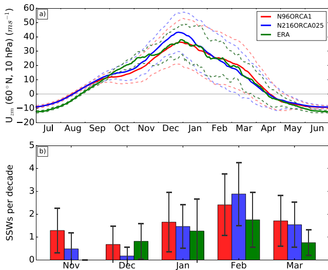
Figure 9. Time series (a) of daily averaged zonally averaged winds ( \text{m/s} ) at 60^\circ\text{N} and 10 hPa. Solid lines indicate the mean wind, and dashed lines indicate the 1 standard deviation range for simulations and the ERA-40 (1958–1978; Uppala et al., 2005) plus ERA-Interim (1979–2018; Dee et al., 2011) reanalyses. Bar chart (b) of number of SSWs per decade from the N96ORCA1 (red) and N216ORCA025 (blue) simulations compared with the reanalyses for the period 1958–2018 (green). Whiskers indicate the 1 standard deviation range. SSW = sudden stratospheric cooling.
