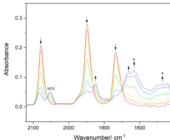
Figure 14. IR SEC monitoring of the reduction of [\text{Mo}(\eta^3\text{-allyl})(\text{CO})_2(4,4'\text{-dmbipy})(\text{NCS})] , 1 ( \downarrow ) at the cathodic wave R1, generating 1^{\cdot-} ( \uparrow ) and five-coordinate [1-A]^- (*) as a weak adduct with THF. Conditions: THF/TBAH, 268 K, cryostated OTTLE cell.
