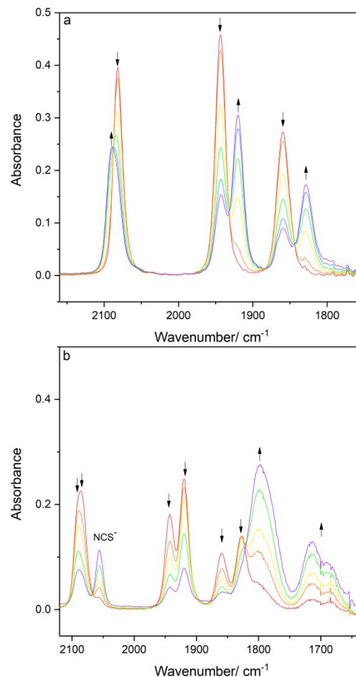
Figure 11. IR SEC monitoring of (a) the initial 1e^- reduction of [\text{Mo}(\eta^3\text{-allyl})(\text{CO})_2(6,6'\text{-dmbipy})(\text{NCS})]^- , 3 ( \downarrow ) at R1 to stable \mathbf{3}^- ( \uparrow ), and (b) the following reduction at R2 showing the conversion of \mathbf{3}^- to [\mathbf{3-A}]^- ( \uparrow ) and free \text{NCS}^- . Conditions: a cryostated OTTLE cell, PrCN/TBAH, 223 K.
