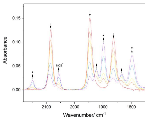
Figure 13. IR SEC monitoring of the electrochemical reduction of [\text{Mo}(\eta^3\text{-allyl})(\text{CO})_2(4,4'\text{-dmbipy})(\text{NCS})] , 1 ( \downarrow ) at the cathodic wave R1, forming 1^{\cdot-} ( \uparrow ) and 6-coordinate [1-\text{PrCN}]^- (*). Conditions: PrCN/TBAH, 223 K, cryostated OTTLE cell.
