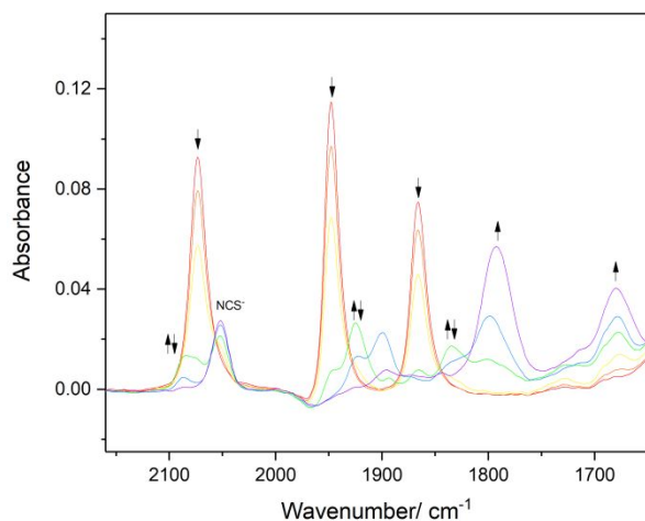
Figure 15. IR SEC monitoring of the initial reduction of [\text{Mo}(\eta^3\text{-allyl})(\text{CO})_2(6,6'\text{-dmbipy})(\text{NCS})] , 3 ( \downarrow ) at R1 to 5-coordinate [\mathbf{3-A}]^- ( \uparrow ) via intermediate \mathbf{3}^{\bullet-} ( \uparrow\downarrow ). Conditions: THF/TBAH, 293 K, OTTLE cell.
