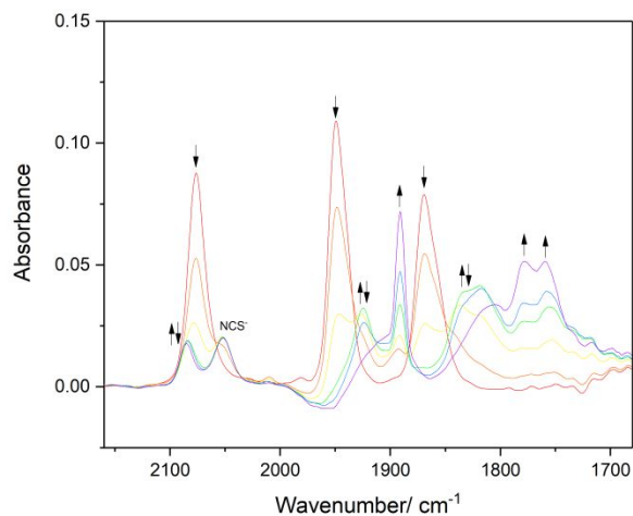
Figure 16. IR SEC monitoring of the 1e^- reduction of [\text{Mo}(\eta^3\text{-allyl})(\text{CO})_2(4,4'\text{-dmbipy})(\text{NCS})] , 1 ( \downarrow ) at R1 to intermediate \mathbf{1}^{\bullet-} ( \downarrow ) concomitantly converting to [\text{Mo}(\eta^3\text{-allyl})(\text{CO})_2(4,4'\text{-dmbipy})]_2 -related dimer [\mathbf{1-D}'] ( \uparrow ). Conditions: THF/TBAH, 293 K, OTTLE cell.
