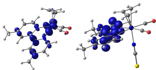
Figure 7. DFT-calculated spin density in the 5-coordinate radical [\text{Mo}(\eta^3\text{-allyl})(\text{CO})_2(4,4'\text{-dmbipy})]^- , [1-R] (left), and precursor 6-coordinate radical anion [1] - (right).
